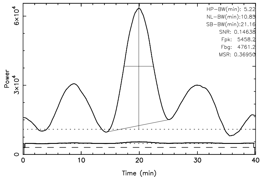
TOYOKAWA 3C123 2024/09/10(254)04:51:42-05:31:42JST
