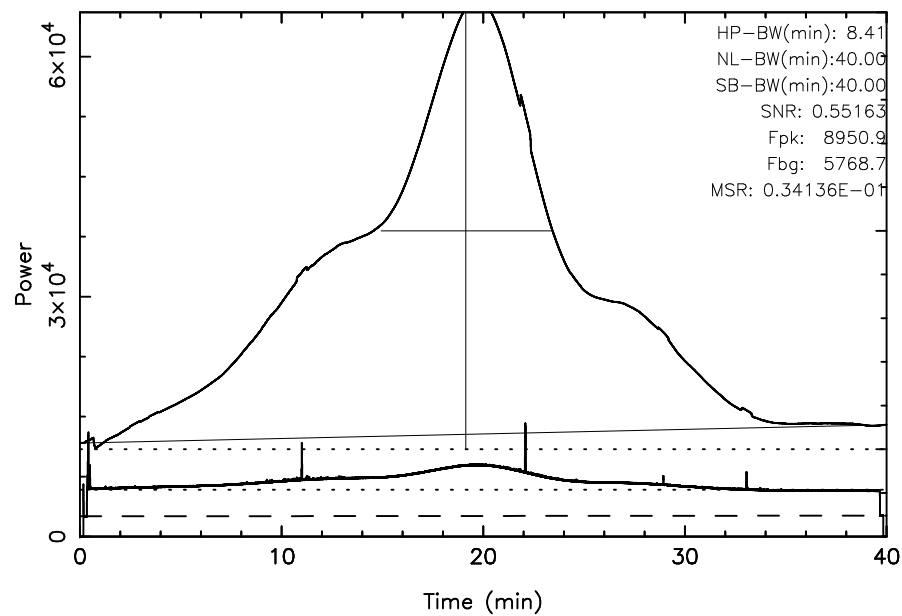
TOYOKAWA 3C392 2024/09/10(254)19:08:04-19:48:04JST
