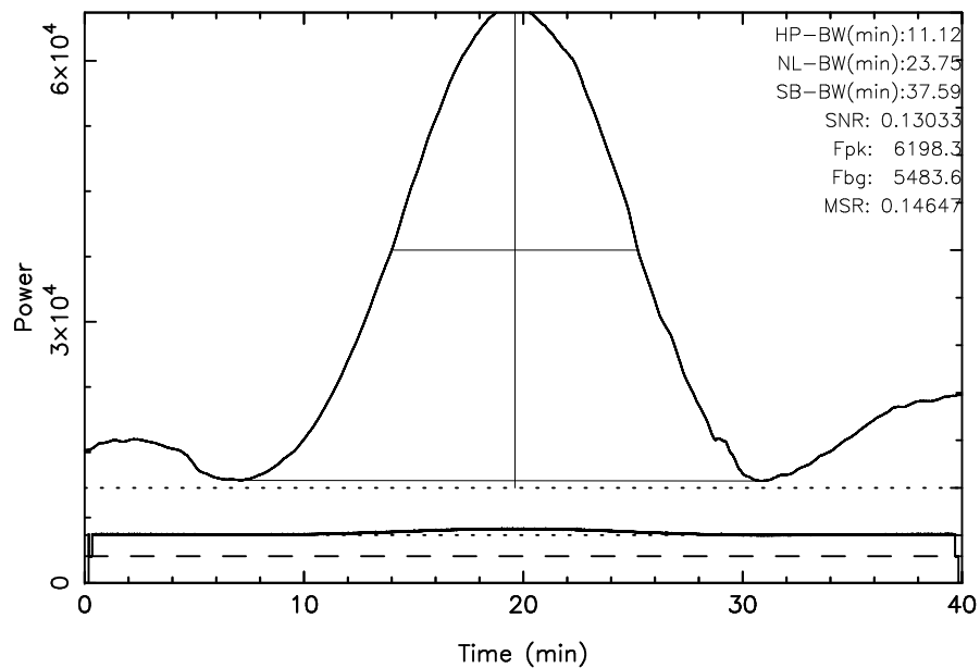
TOYOKAWA 3C10 2024/09/10(254)00:40:33-01:20:33JST
