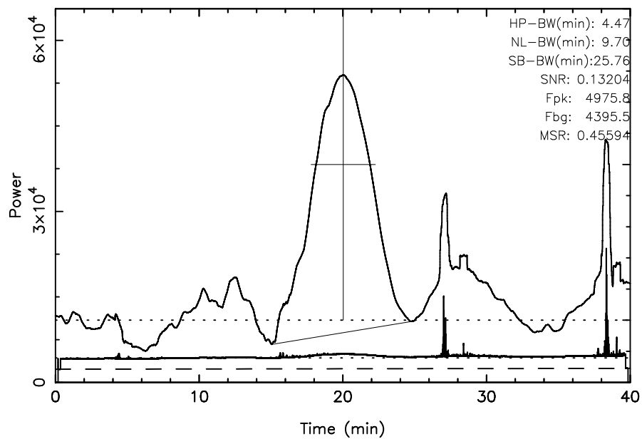
TOYOKAWA 3C353 2024/09/10(254)17:32:46-18:12:46JST
