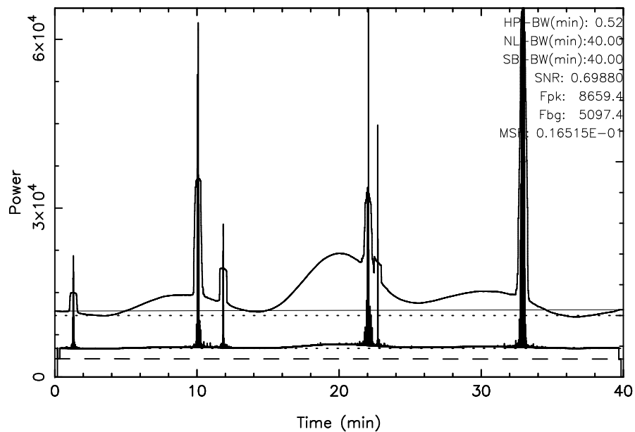
TOYOKAWA 3C123 2024/09/24(268)03:56:39-04:36:39JST
