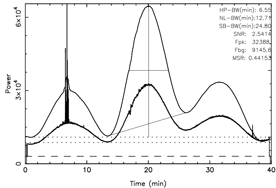
TOYOKAWA 3C405 2024/09/24(268)19:15:50-19:55:50JST
