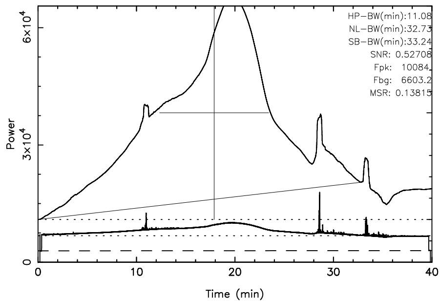
TOYOKAWA 3C392 2024/09/24(268)18:13:01-18:53:01JST
