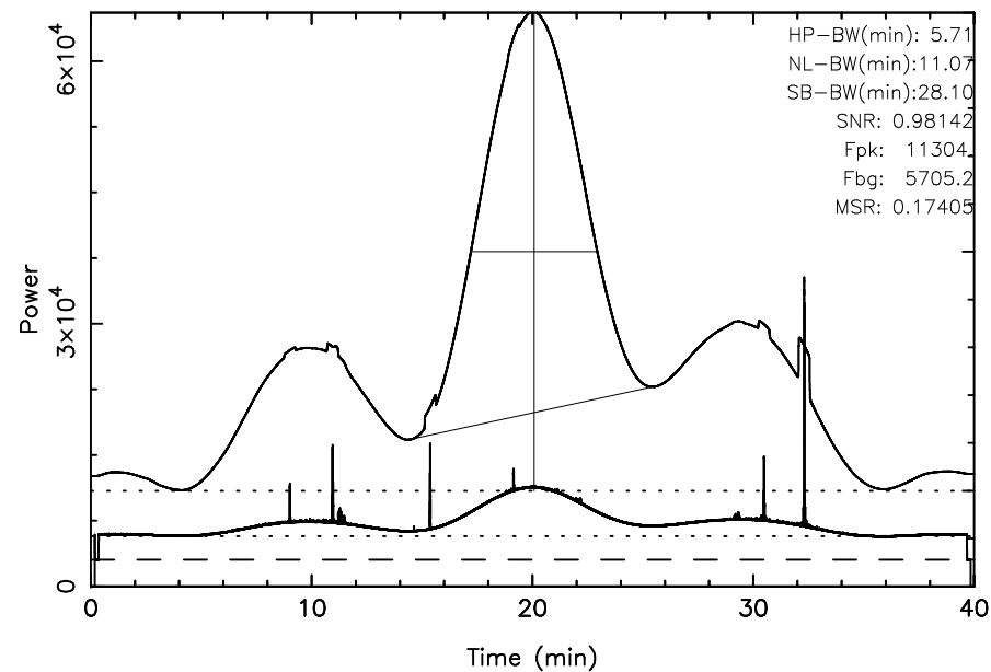
TOYOKAWA 3C144 2024/09/24(268)04:53:52-05:33:52JST
