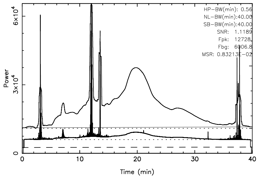
TOYOKAWA 3C392 2024/09/27(271)18:01:14-18:41:14JST
