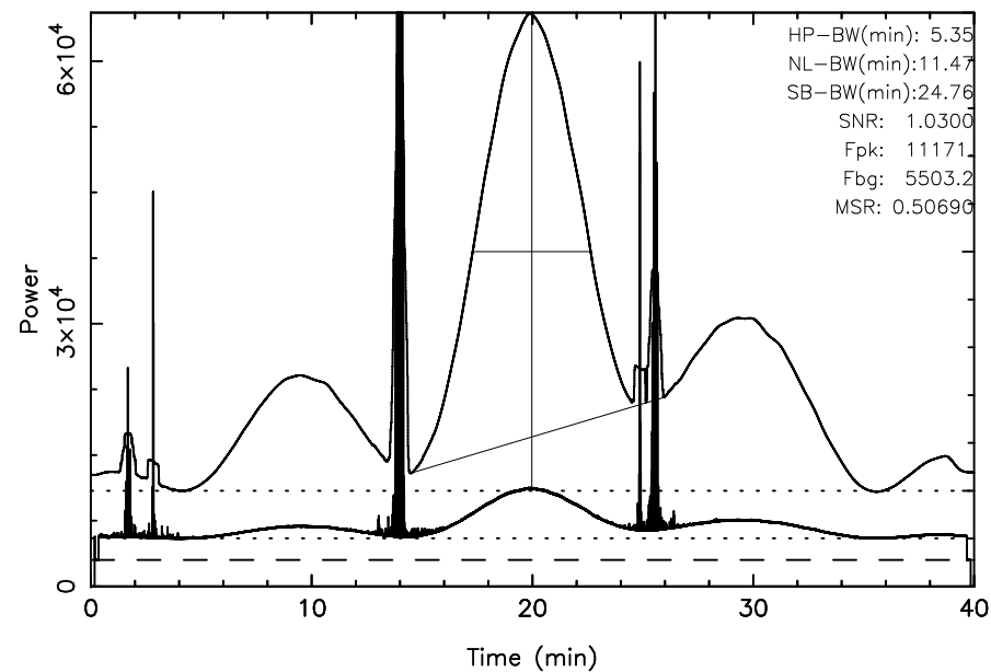
TOYOKAWA 3C144 2024/09/27(271)04:42:04-05:22:04JST
