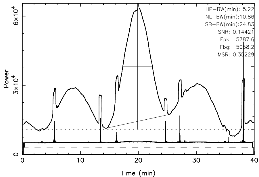
TOYOKAWA 3C123 2024/09/27(271)03:44:52-04:24:52JST
