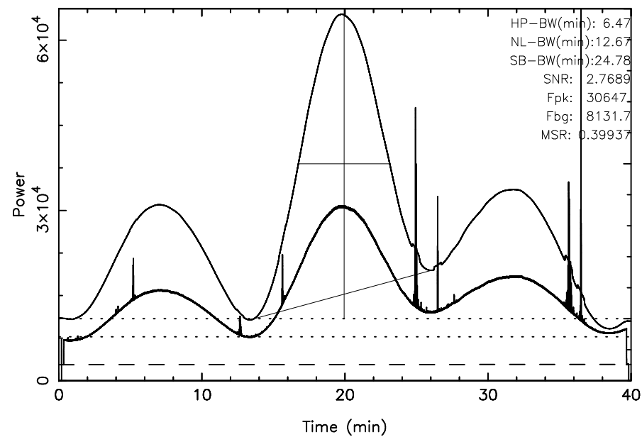
TOYOKAWA 3C405 2024/09/27(271)19:04:02-19:44:02JST
