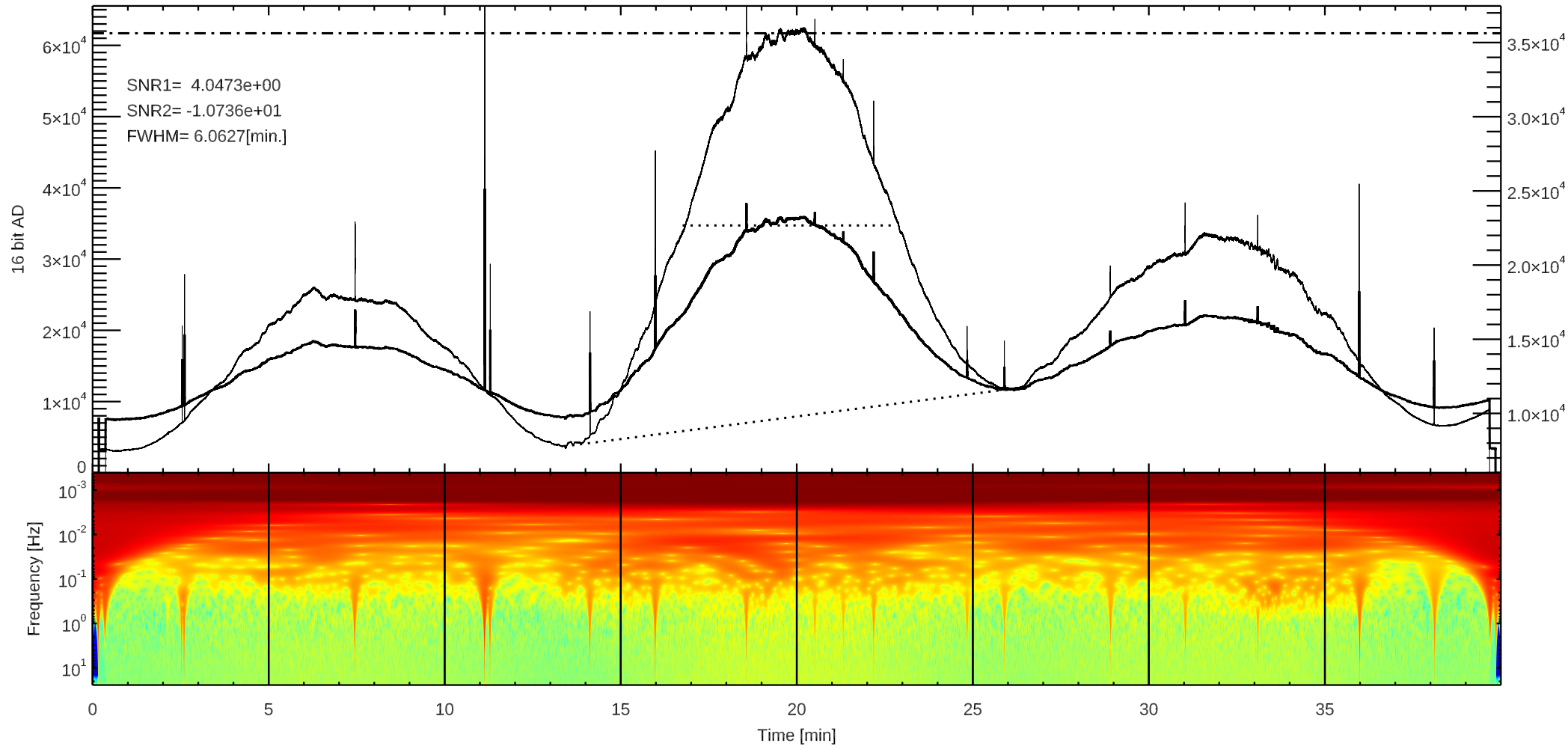
C 3C405 (/home4/archive/swift/dat/2024/10/T20241007182445.dat)
