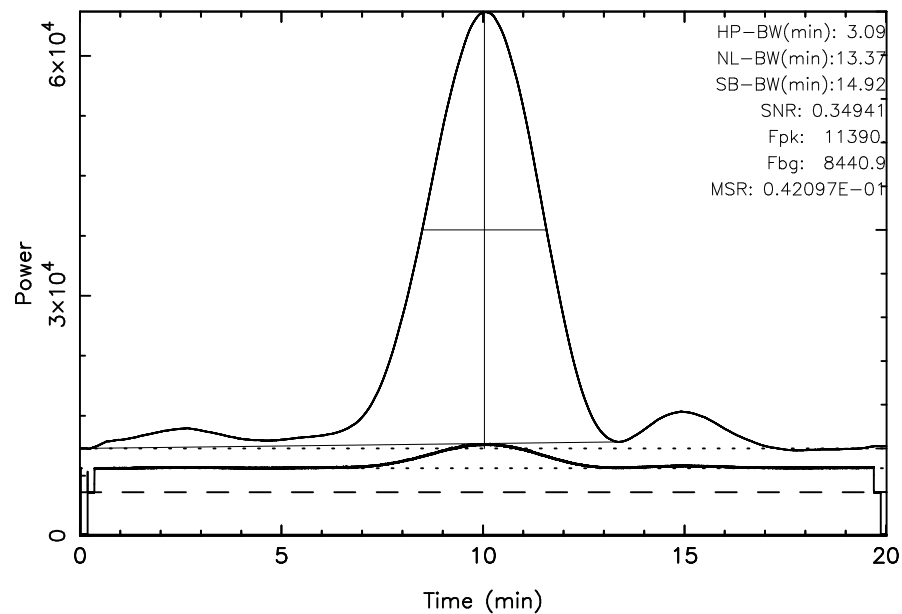
KISO 3C144 2024/10/08(282)04:08:48-04:28:49JST
