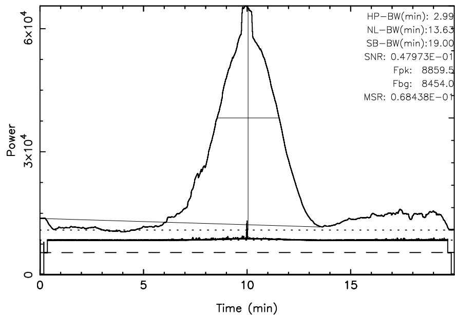
KISO 3C123 2024/10/08(282)03:11:37-03:31:37JST
