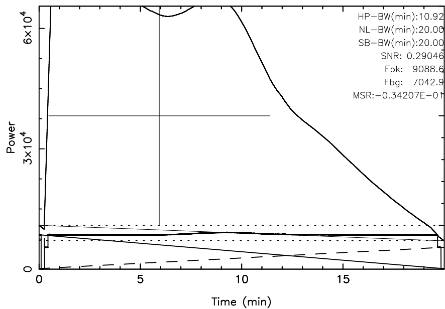
KISO 3C157 2024/10/08(282)04:52:14-05:12:14JST
