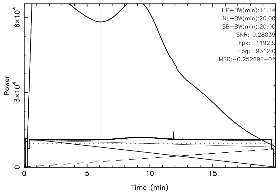
KISO 3C157 2024/10/10(284)04:44:21-05:04:21JST
