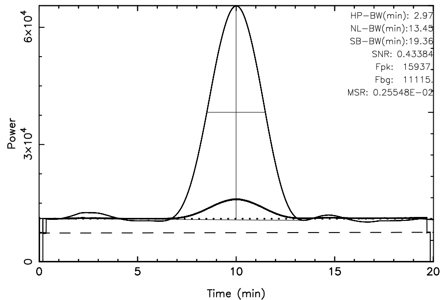
KISO 3C144 2024/10/10(284)04:00:57-04:20:58JST
