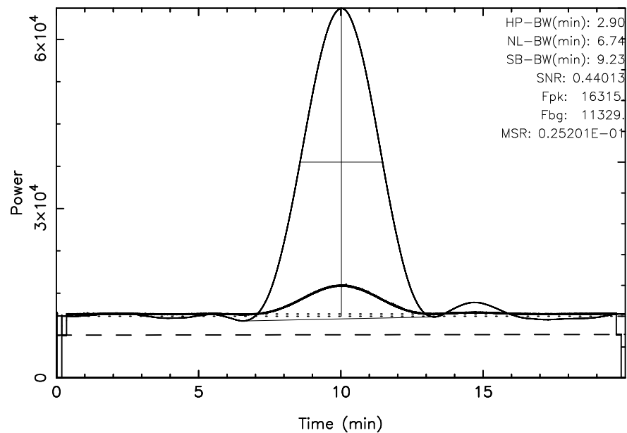
KISO 3C144 2024/10/11(285)03:57:02-04:17:02JST
