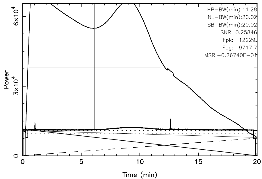
KISO 3C157 2024/10/11(285)04:40:25-05:00:26JST
