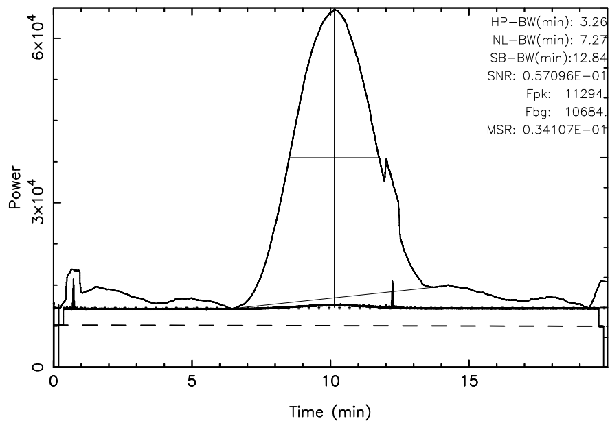
KISO 3C123 2024/10/11(285)02:59:48-03:19:48JST
