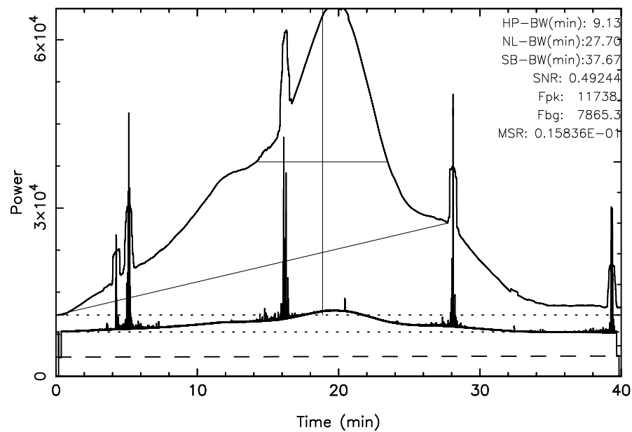
TOYOKAWA 3C392 2024/10/02(276)17:41:34-18:21:34JST
