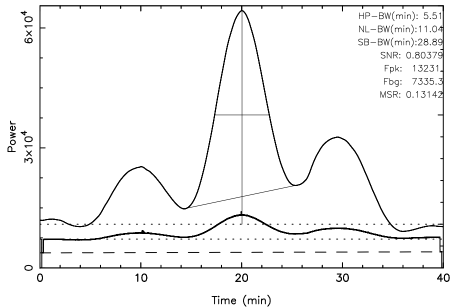
TOYOKAWA 3C144 2024/10/02(276)04:22:25-05:02:25JST
