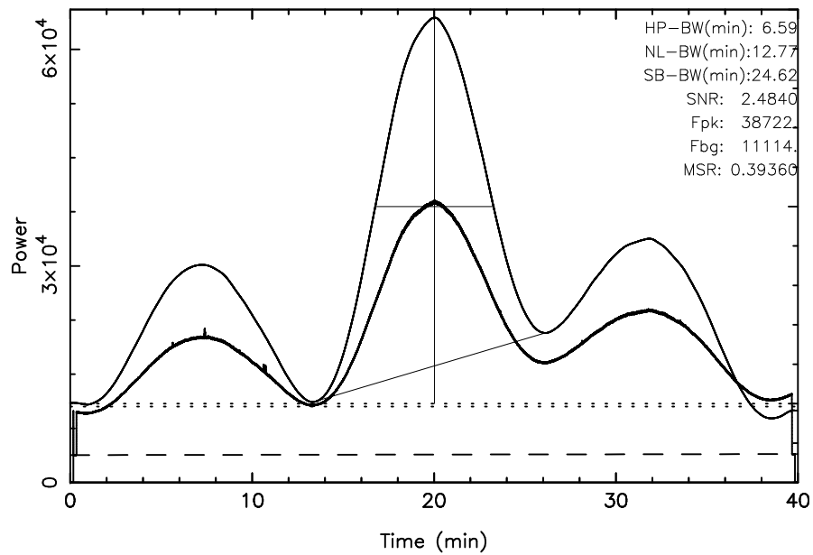
TOYOKAWA 3C405 2024/10/02(276)18:44:22-19:24:22JST
