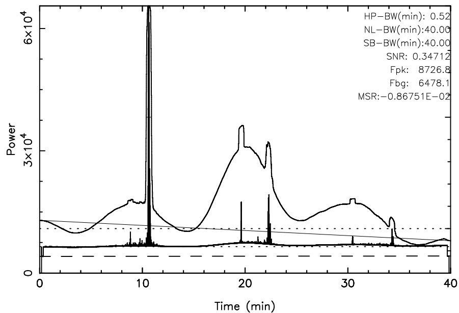
TOYOKAWA 3C123 2024/10/02(276)03:25:12-04:05:12JST
