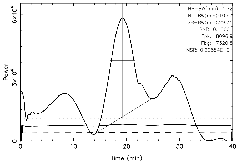
TOYOKAWA 3C157 2024/10/02(276)05:05:49-05:45:49JST
