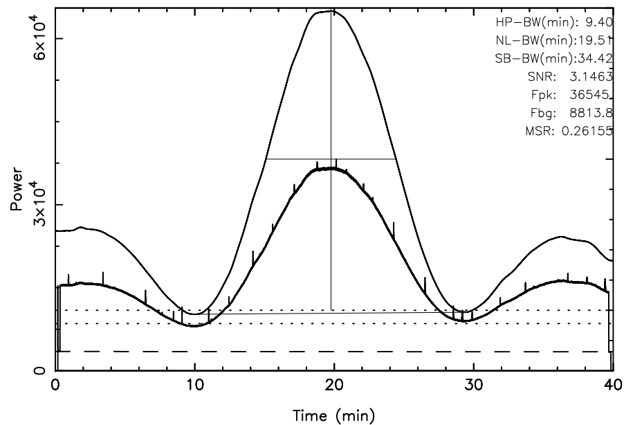
TOYOKAWA 3C461 2024/10/05(279)21:56:11-22:36:11JST
