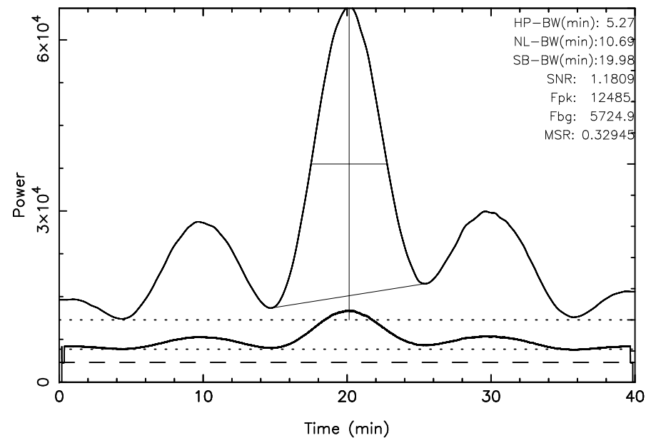
TOYOKAWA 3C144 2024/10/05(279)04:10:37-04:50:37JST
