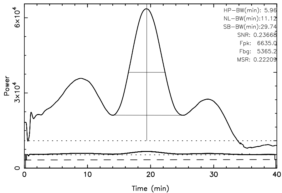
TOYOKAWA 3C157 2024/10/05(279)04:54:01-05:34:01JST
