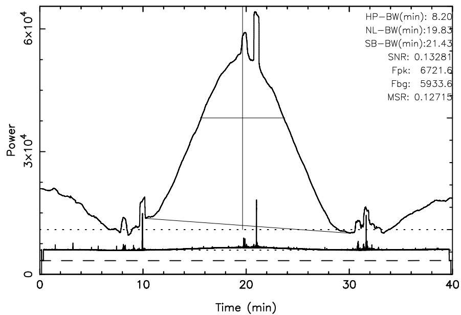
TOYOKAWA 3C10 2024/10/05(279)22:58:20-23:38:20JST
