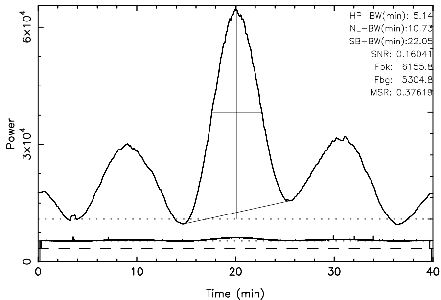
TOYOKAWA 3C123 2024/10/05(279)03:13:24-03:53:24JST
