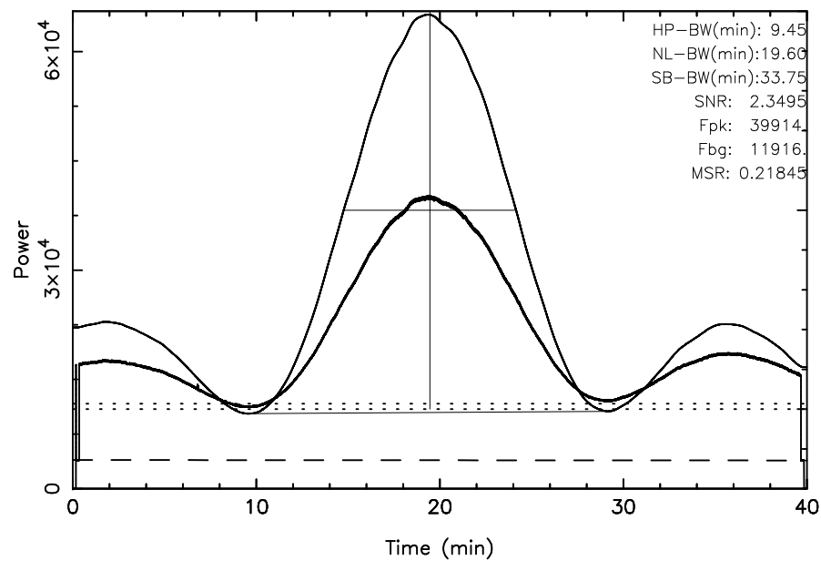
TOYOKAWA 3C461 2024/10/22(296)20:49:21-21:29:21JST
