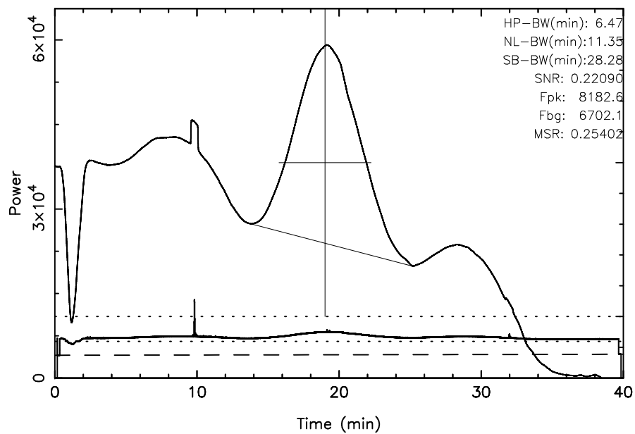
TOYOKAWA 3C157 2024/10/22(296)03:47:11-04:27:11JST
