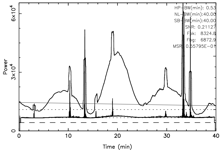
TOYOKAWA 3C123 2024/10/22(296)02:06:34-02:46:34JST
