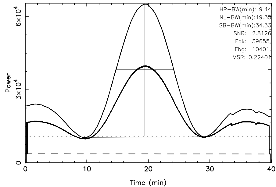
TOYOKAWA 3C461 2024/10/24(298)20:41:29-21:21:29JST
