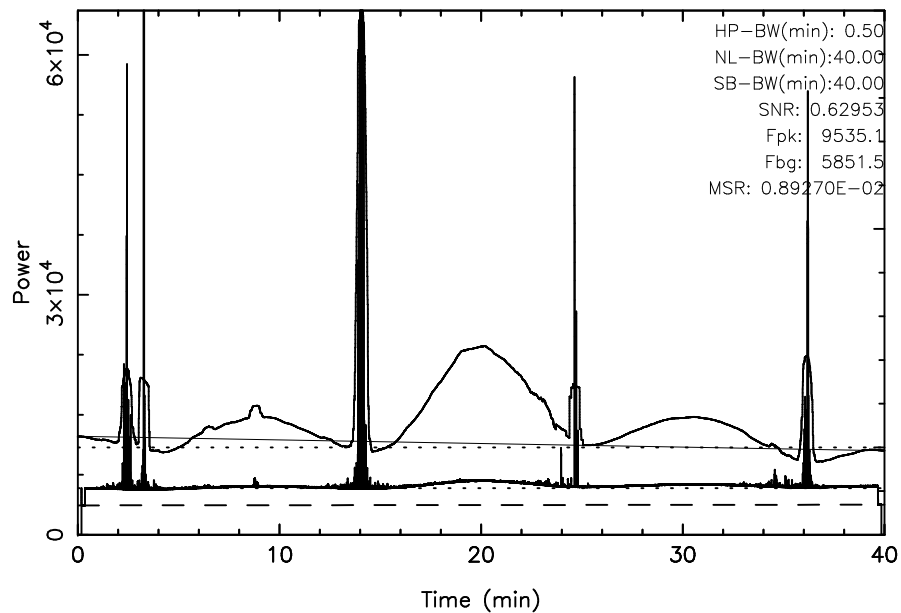
TOYOKAWA 3C123 2024/10/24(298)01:58:42-02:38:42JST
