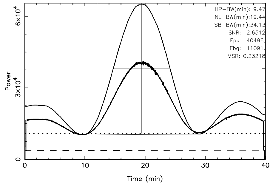
TOYOKAWA 3C461 2024/10/26(300)20:33:37-21:13:37JST
