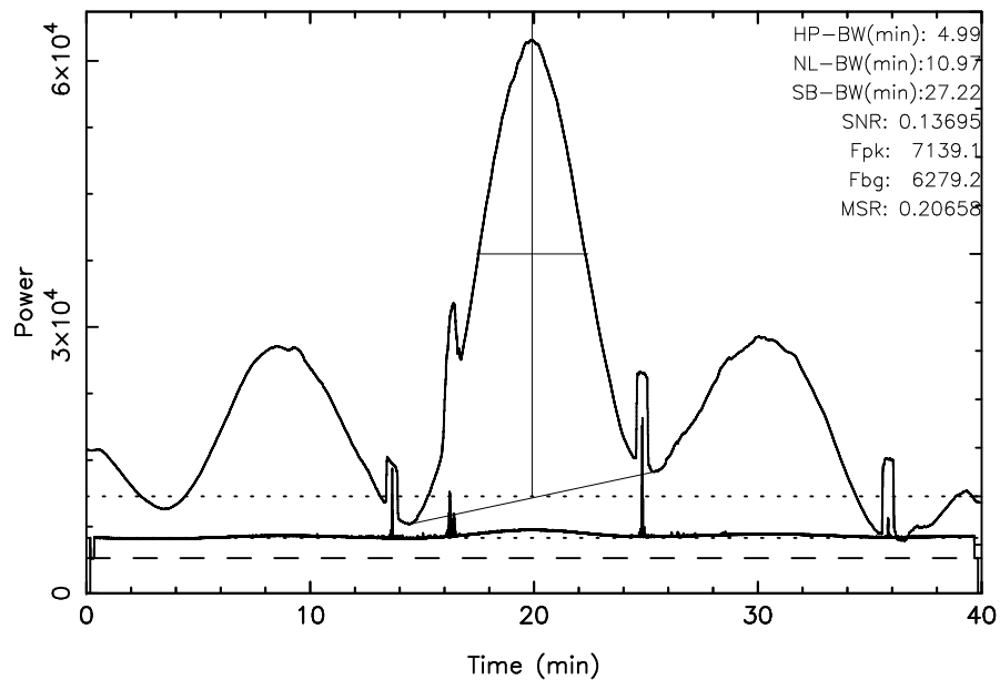
TOYOKAWA 3C123 2024/10/26(300)01:50:51-02:30:51JST
