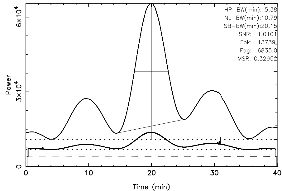
TOYOKAWA 3C144 2024/10/26(300)02:48:03-03:28:03JST
