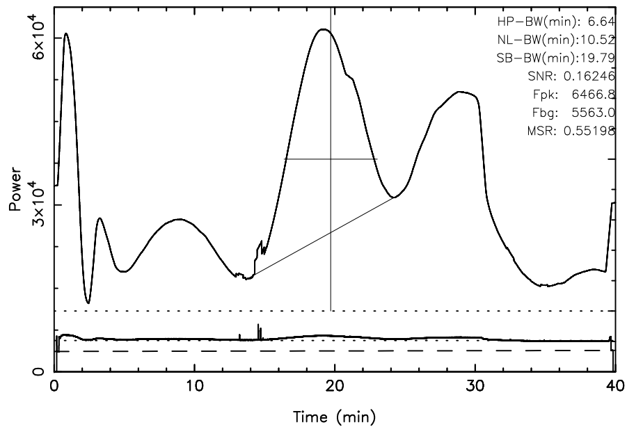
TOYOKAWA 3C157 2024/10/26(300)03:31:27-04:11:27JST
