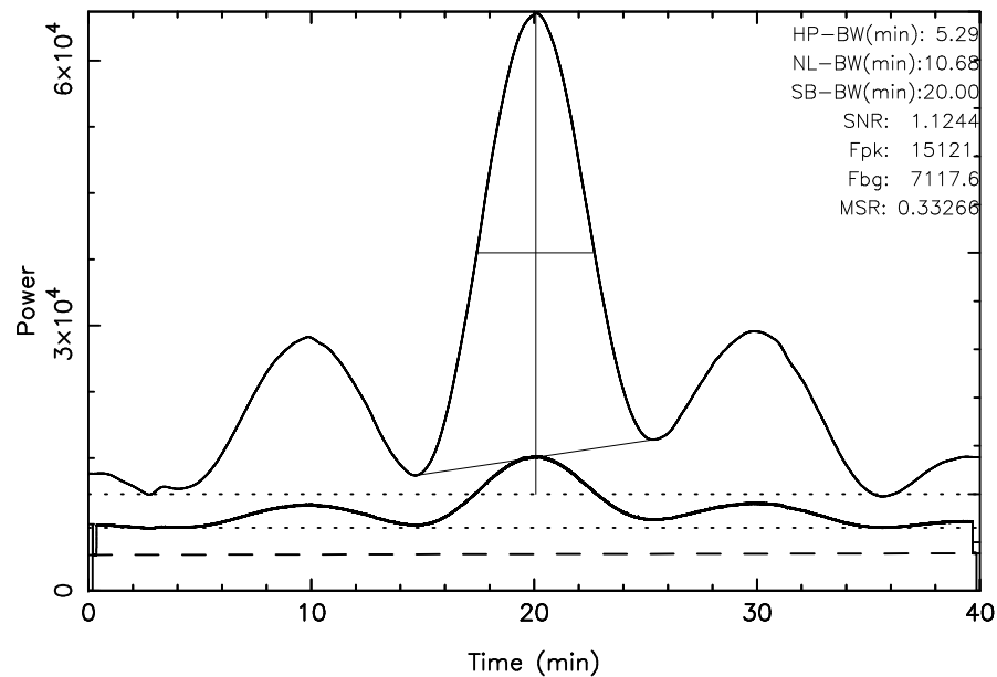
TOYOKAWA 3C144 2024/10/30(304)02:32:20-03:12:20JST
