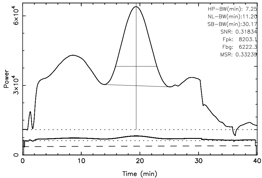
TOYOKAWA 3C157 2024/10/30(304)03:15:44-03:55:44JST
