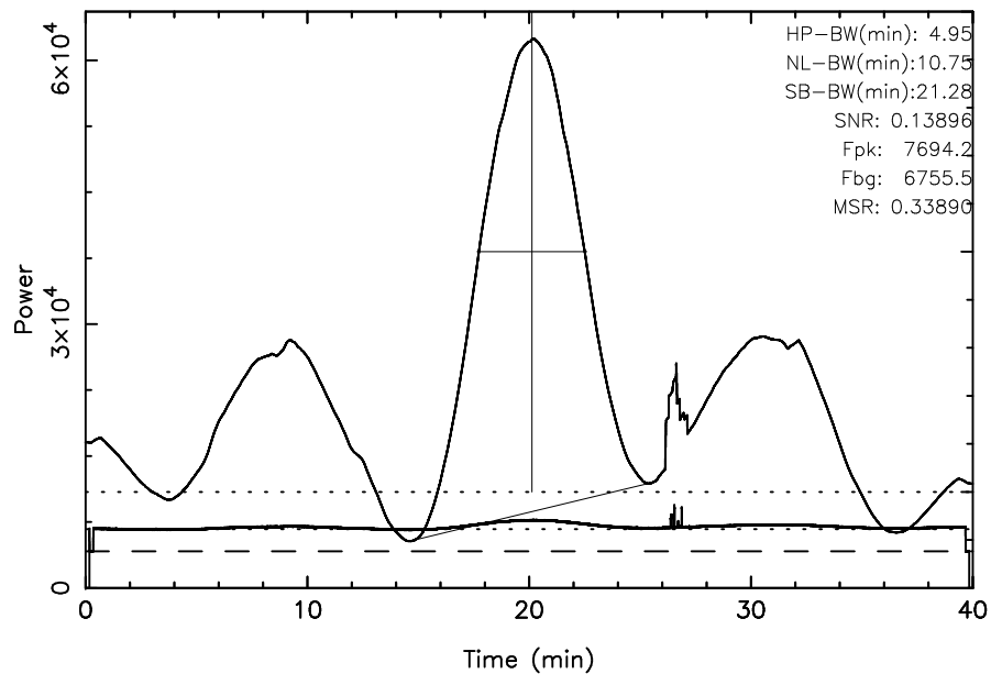
TOYOKAWA 3C123 2024/10/30(304)01:35:07-02:15:07JST
