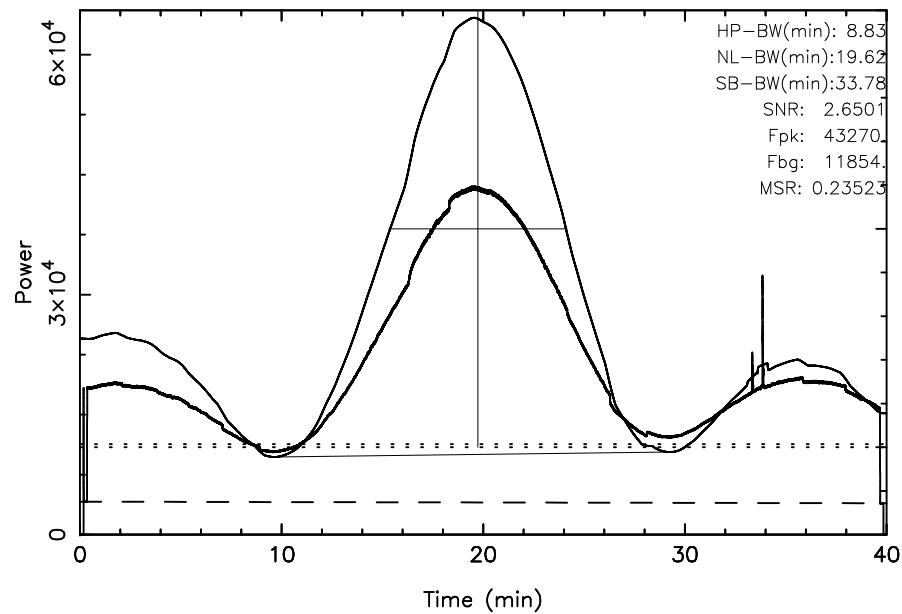
TOYOKAWA 3C461 2024/10/30(304)20:17:54-20:57:54JST
