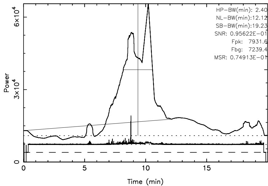
FUJI 3C157 2024/11/14(319)02:26:45-02:46:44JST
