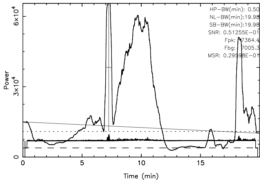
FUJI 3C123 2024/11/14(319)00:46:08-01:06:07JST
