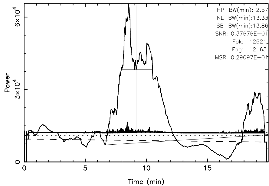
KISO 3C123 2024/11/14(319)00:46:08-01:06:07JST
