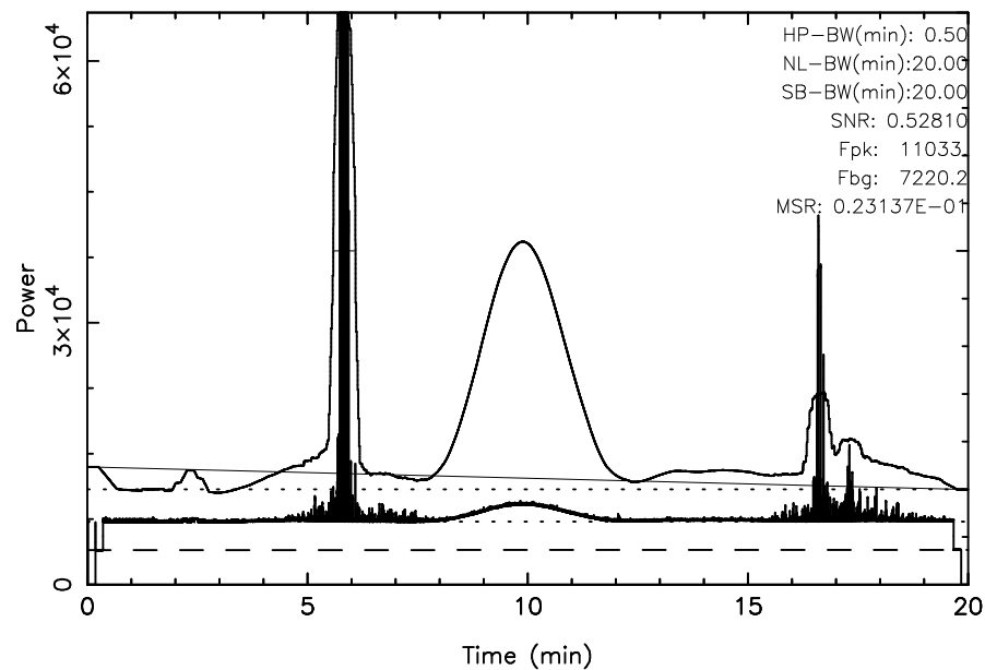
FUJI 3C144 2024/11/14(319)01:43:20-02:03:20JST
