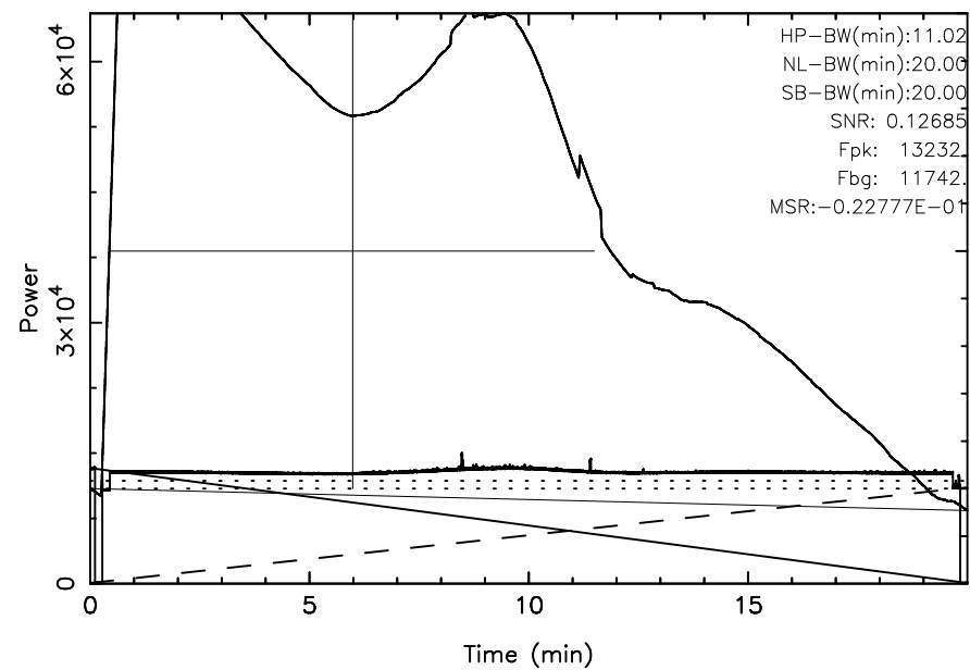
KISO 3C157 2024/11/28(333)01:31:42-01:51:42JST
