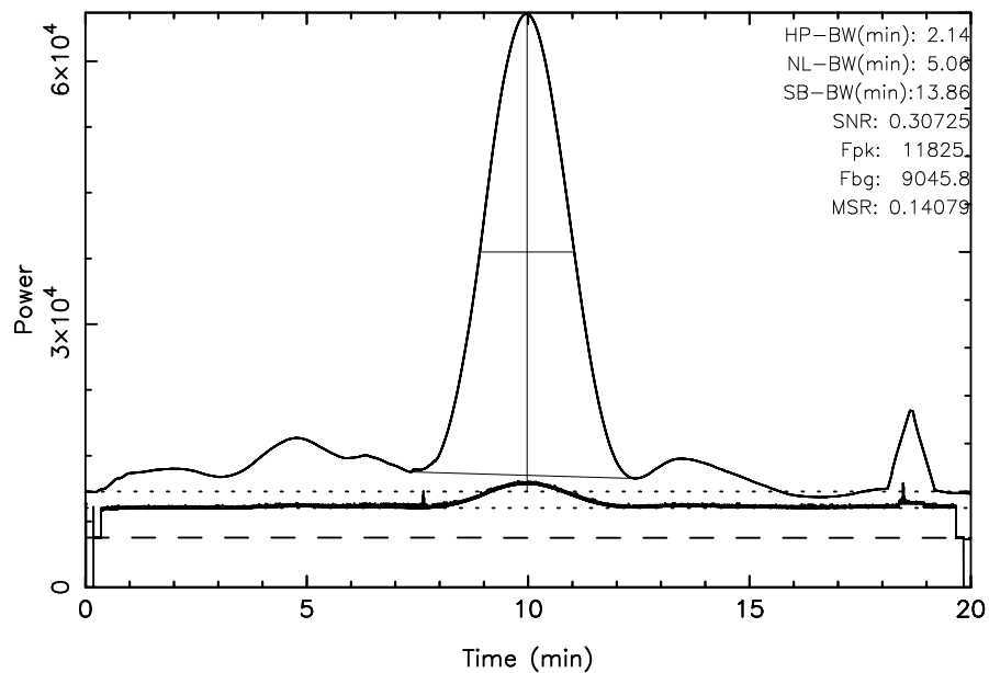
FUJI 3C144 2024/11/28(333)00:48:18-01:08:18JST
