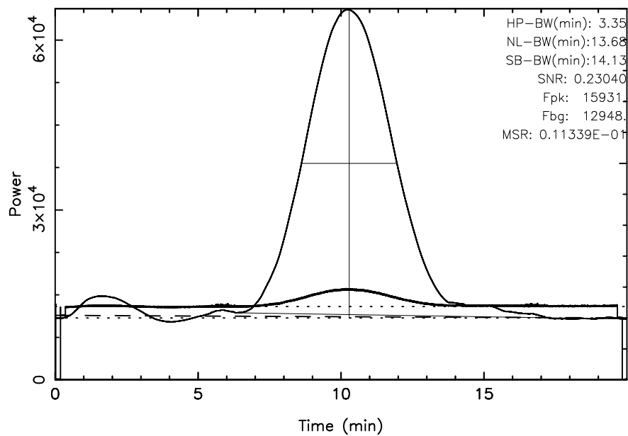
KISO 3C144 2024/11/28(333)00:48:18-01:08:18JST
