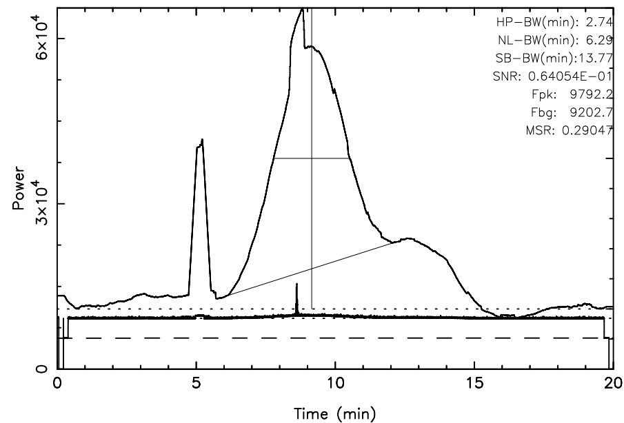
FUJI 3C157 2024/11/28(333)01:31:42-01:51:42JST
