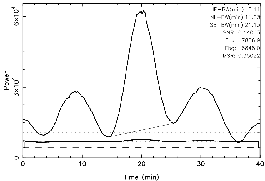
TOYOKAWA 3C123 2024/11/01(306)01:27:15-02:07:15JST
