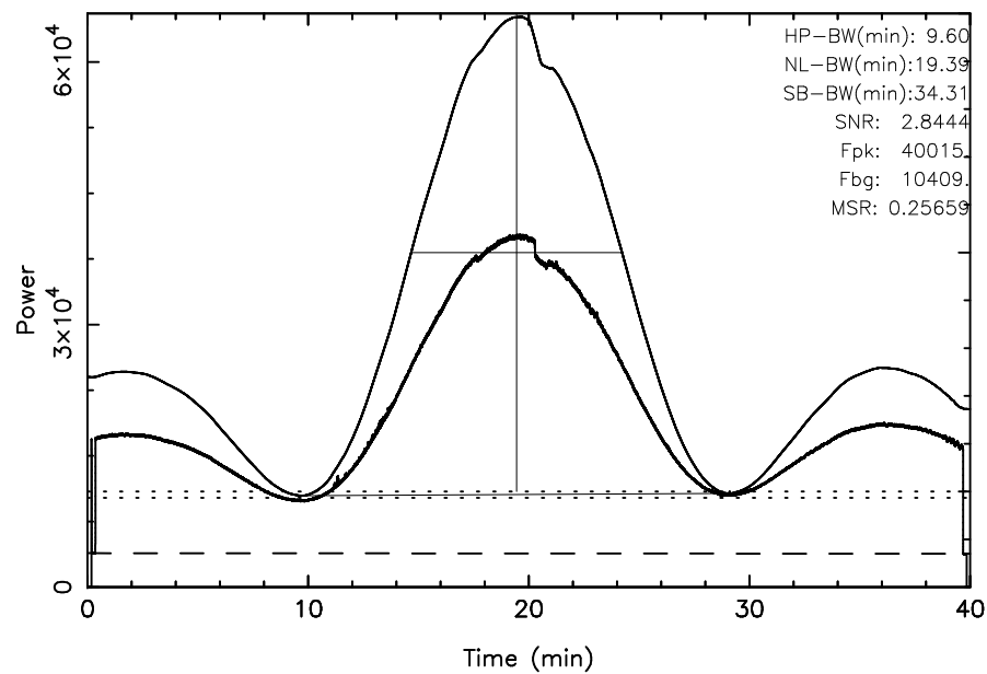
TOYOKAWA 3C461 2024/11/01(306)20:10:02-20:50:02JST
