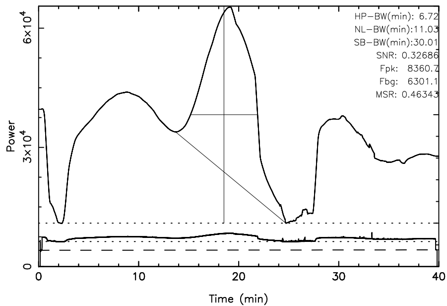
TOYOKAWA 3C157 2024/11/01(306)03:07:52-03:47:52JST
