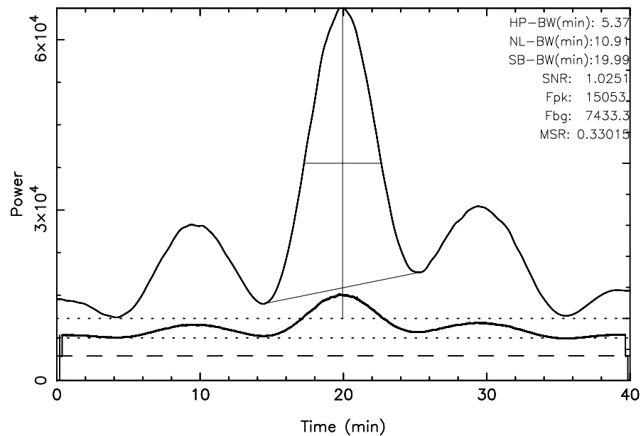
TOYOKAWA 3C144 2024/11/01(306)02:24:28-03:04:28JST
