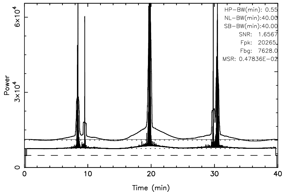
TOYOKAWA 3C123 2024/11/12(317)00:44:00-01:24:00JST
