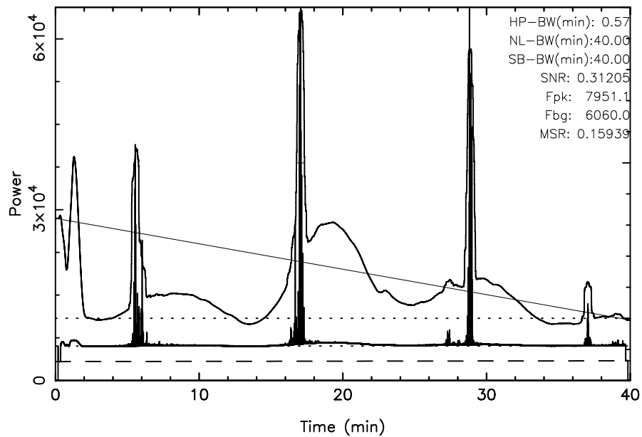
TOYOKAWA 3C157 2024/11/12(317)02:24:37-03:04:37JST
