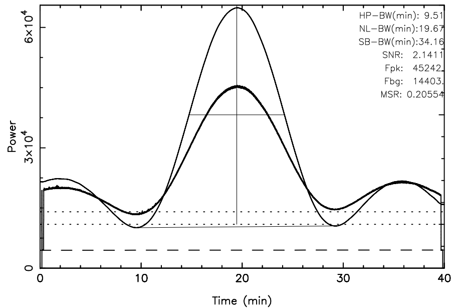
TOYOKAWA 3C461 2024/11/12(317)19:26:47-20:06:47JST
