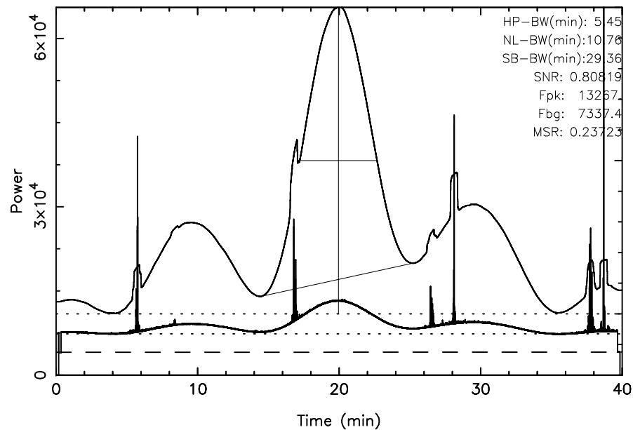
TOYOKAWA 3C144 2024/11/12(317)01:41:13-02:21:13JST
