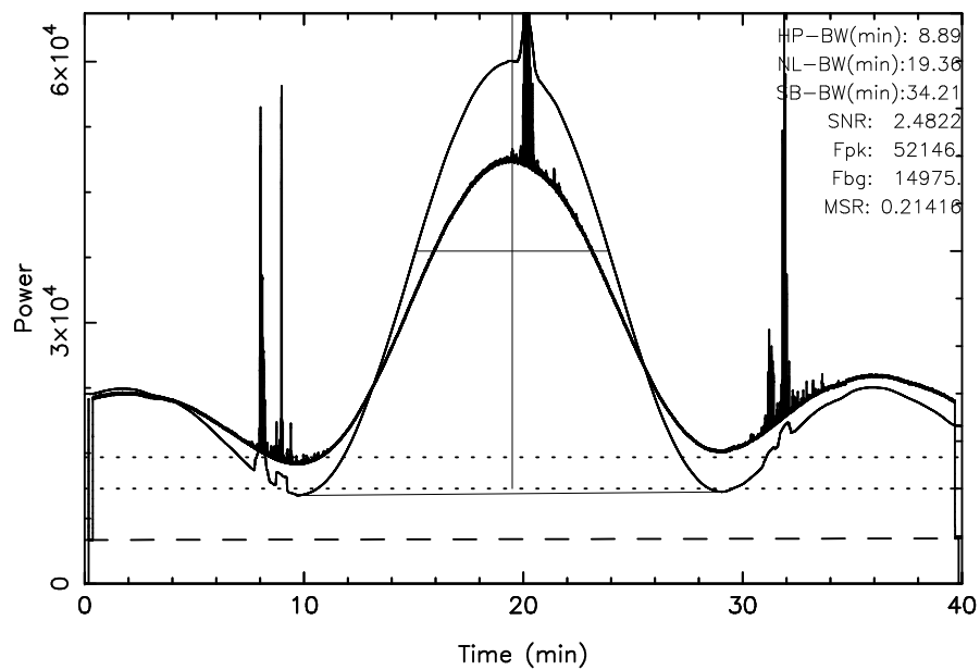
TOYOKAWA 3C461 2024/11/27(332)18:27:48-19:07:48JST
