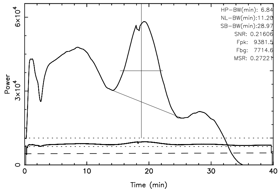
TOYOKAWA 3C157 2024/11/27(332)01:25:39-02:05:39JST
