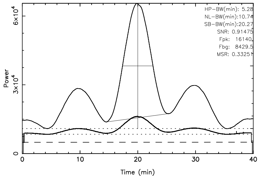
TOYOKAWA 3C144 2024/11/27(332)00:42:14-01:22:14JST
