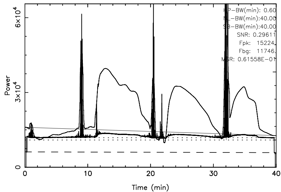
TOYOKAWA 3C10 2024/11/30(335)19:18:09-19:58:09JST
