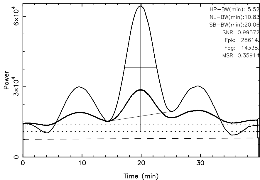
TOYOKAWA 3C144 2024/11/30(335)00:30:27-01:10:27JST
