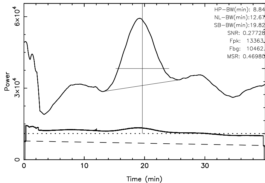
TOYOKAWA 3C157 2024/11/30(335)01:13:51-01:53:51JST
