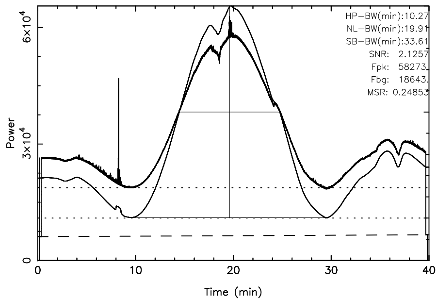
TOYOKAWA 3C461 2024/11/30(335)18:16:01-18:56:01JST
