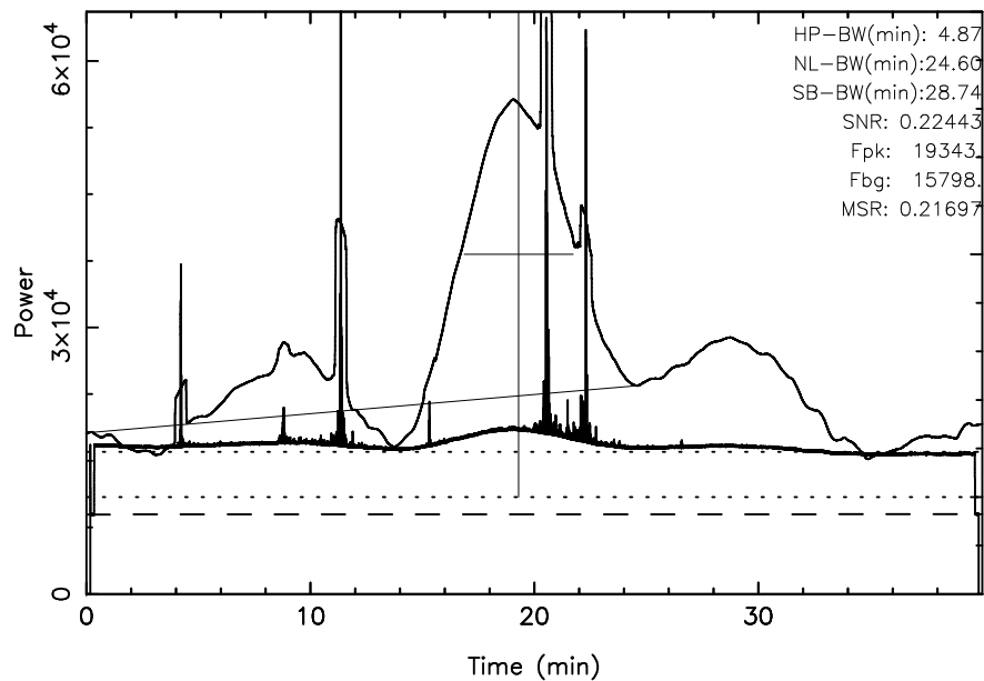
TOYOKAWA 3C157 2024/12/09(344)00:38:28-01:18:28JST
