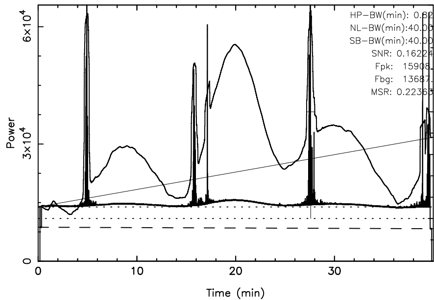
TOYOKAWA 3C123 2024/12/09(344)22:53:55-23:33:55JST
