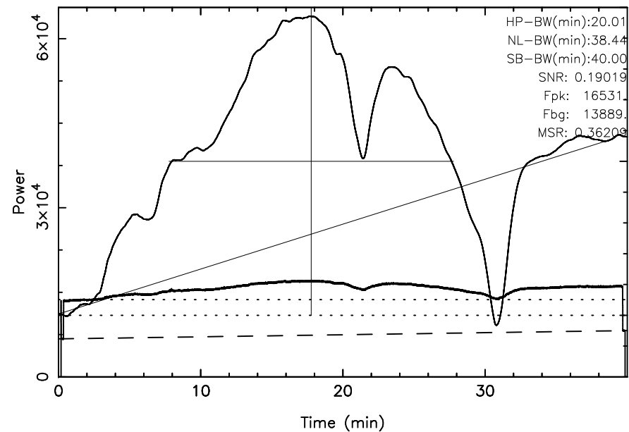
TOYOKAWA 3C10 2024/12/09(344)18:42:46-19:22:46JST
