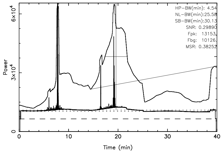
TOYOKAWA 3C123 2024/12/17(352)22:22:28-23:02:28JST
