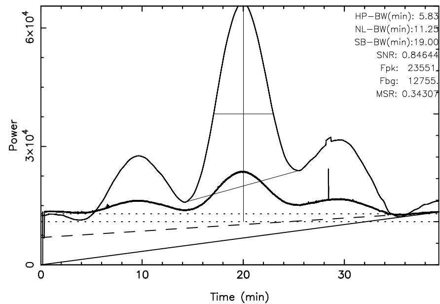
TOYOKAWA 3C144 2024/12/17(352)23:19:40-23:59:40JST
