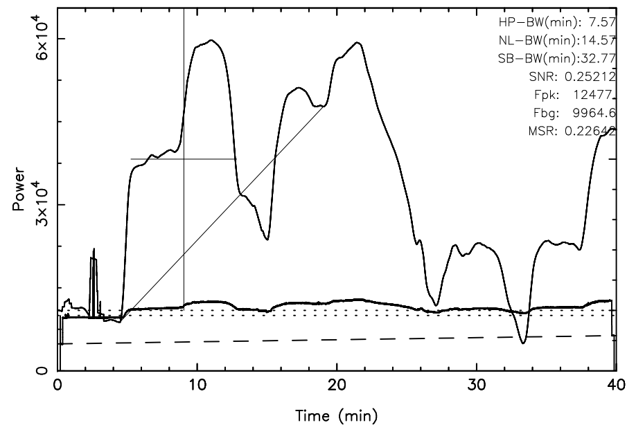
TOYOKAWA 3C10 2024/12/17(352)18:11:19-18:51:19JST
