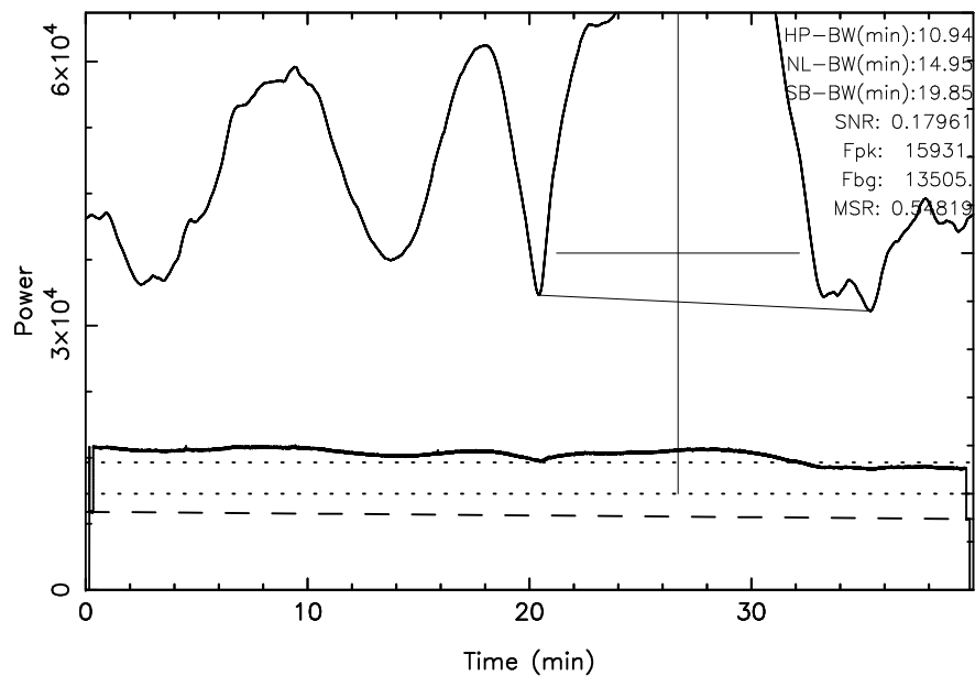
TOYOKAWA 3C157 2024/12/17(352)00:07:01-00:47:01JST
