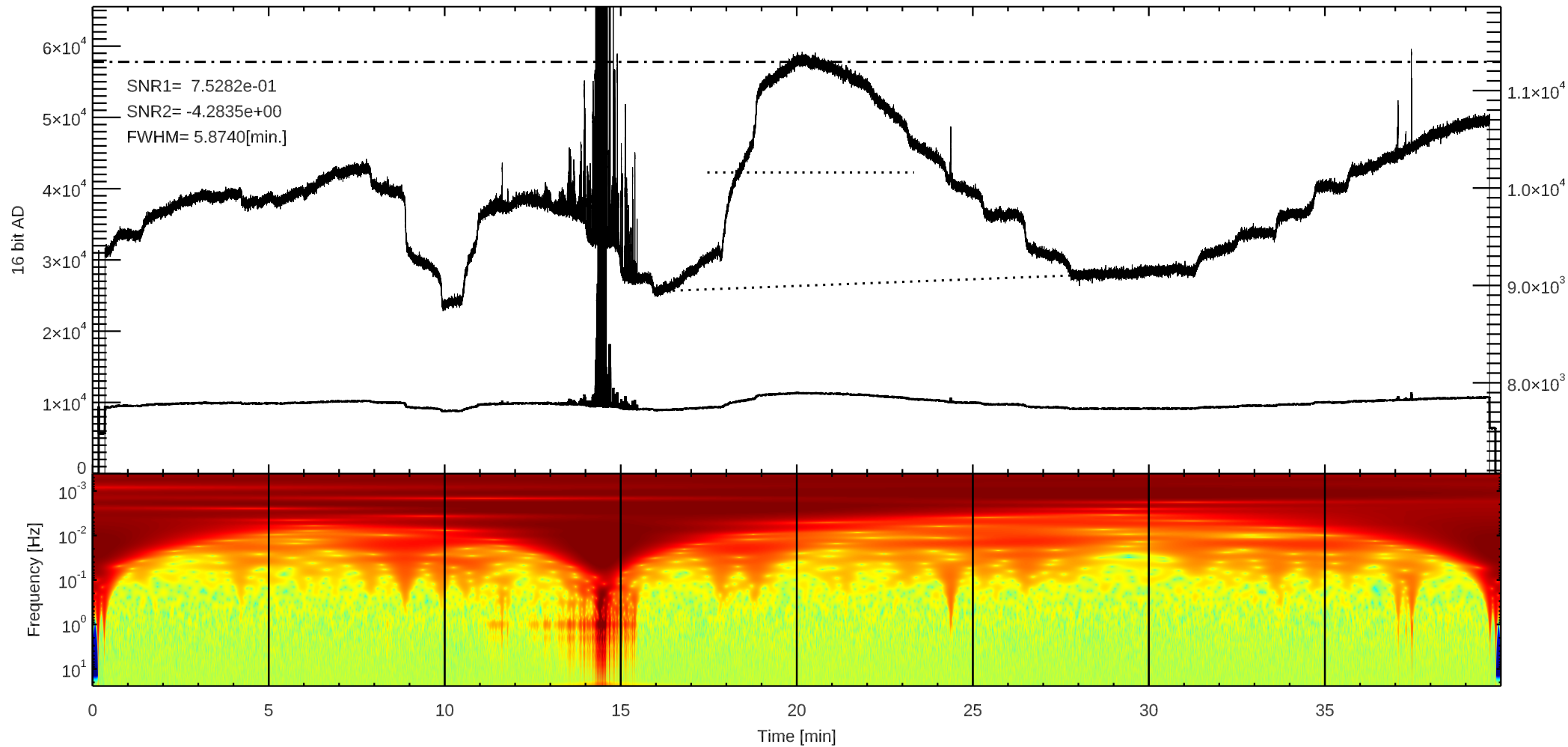
C 3C123 (/home4/archive/swift/dat/2025/01/T20250126194514.dat)
