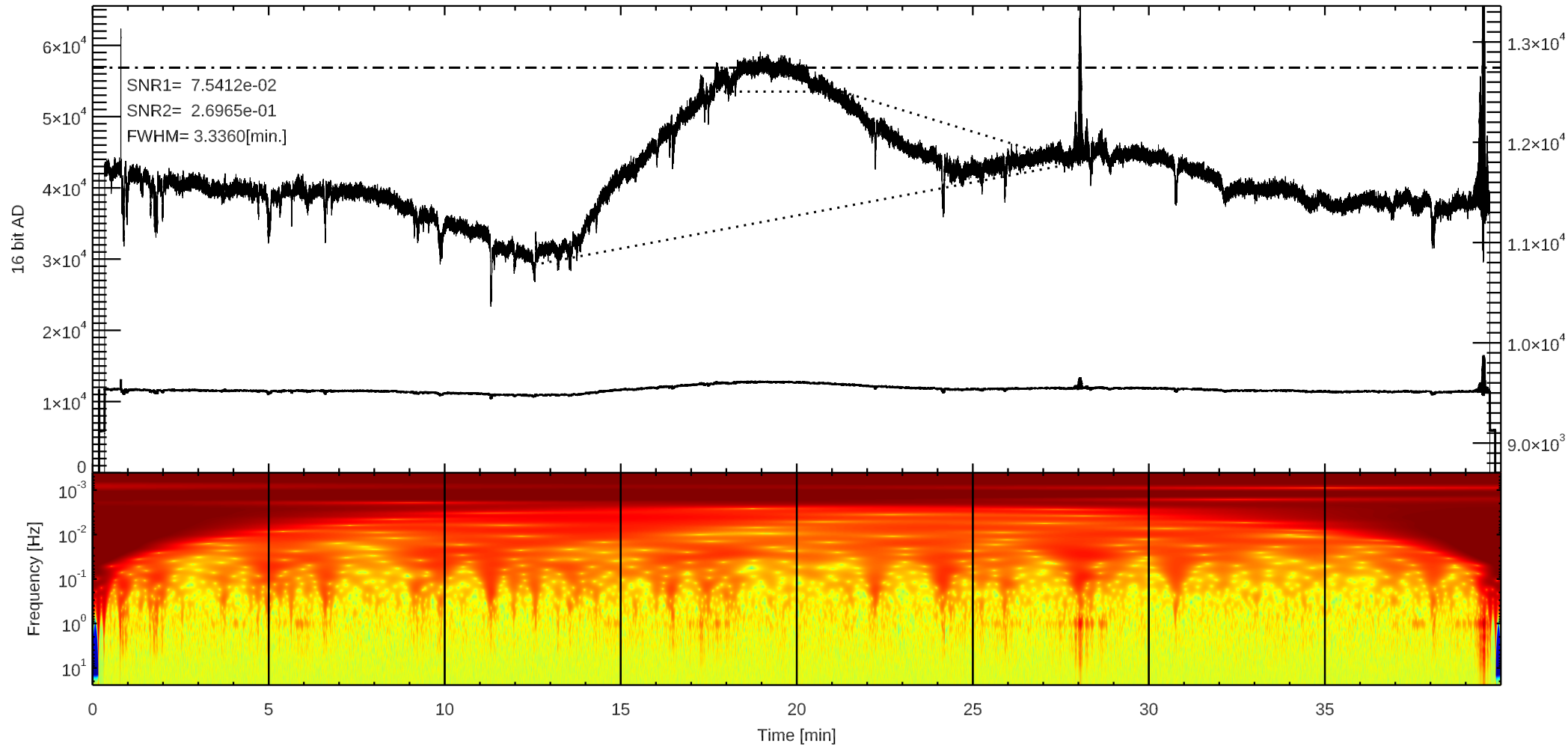
C 3C157 (/home4/archive/swift/dat/2025/01/T20250117220114.dat)
