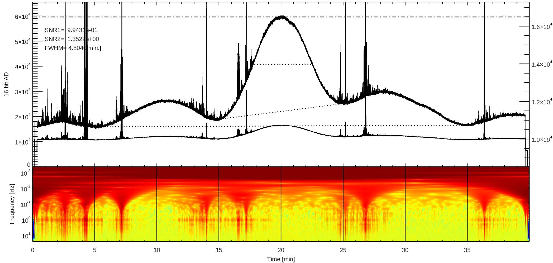
C 3C274 (/home4/archive/swift/dat/2025/01/T20250105050352.dat)
