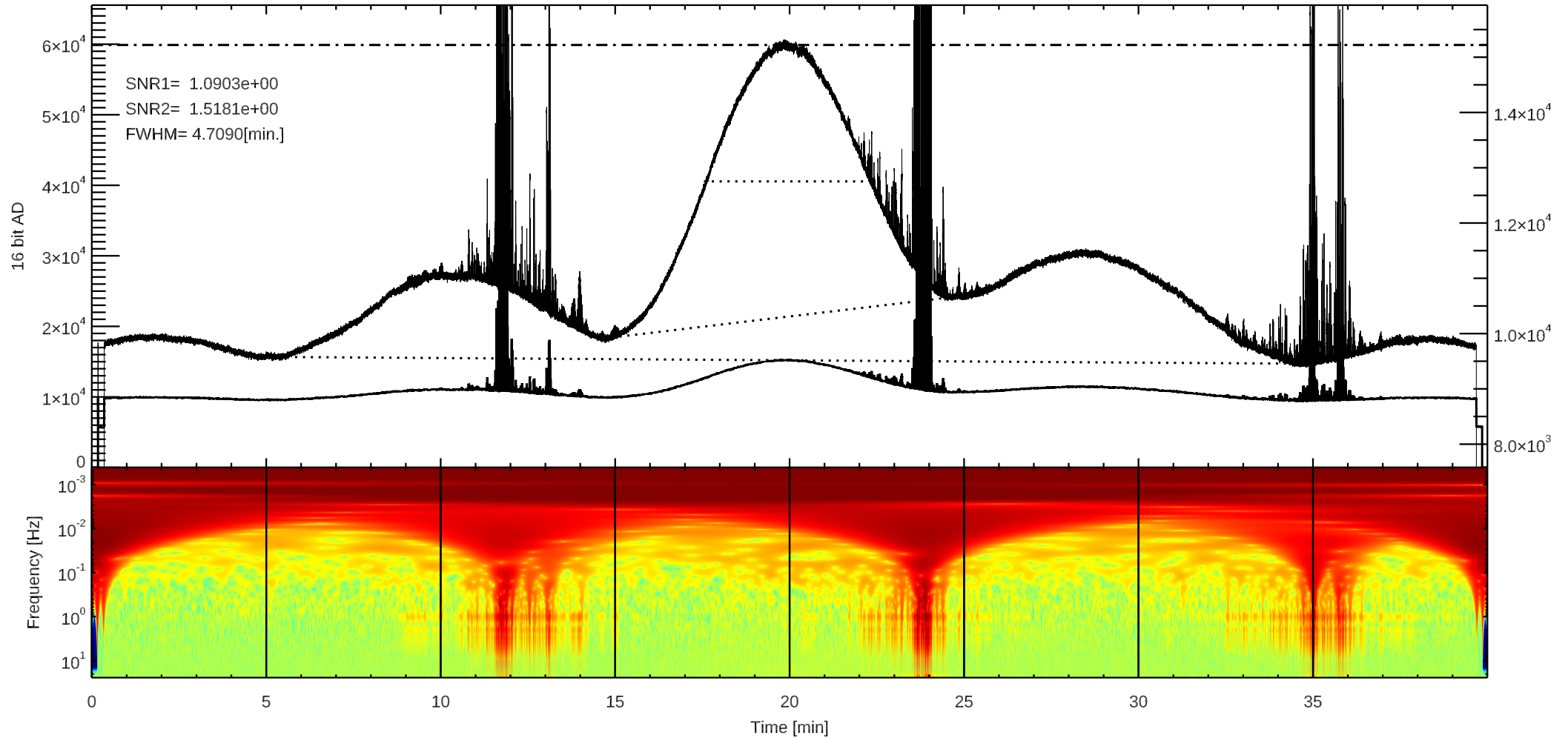
C 3C274 (/home4/archive/swift/dat/2025/01/T20250131032139.dat)
