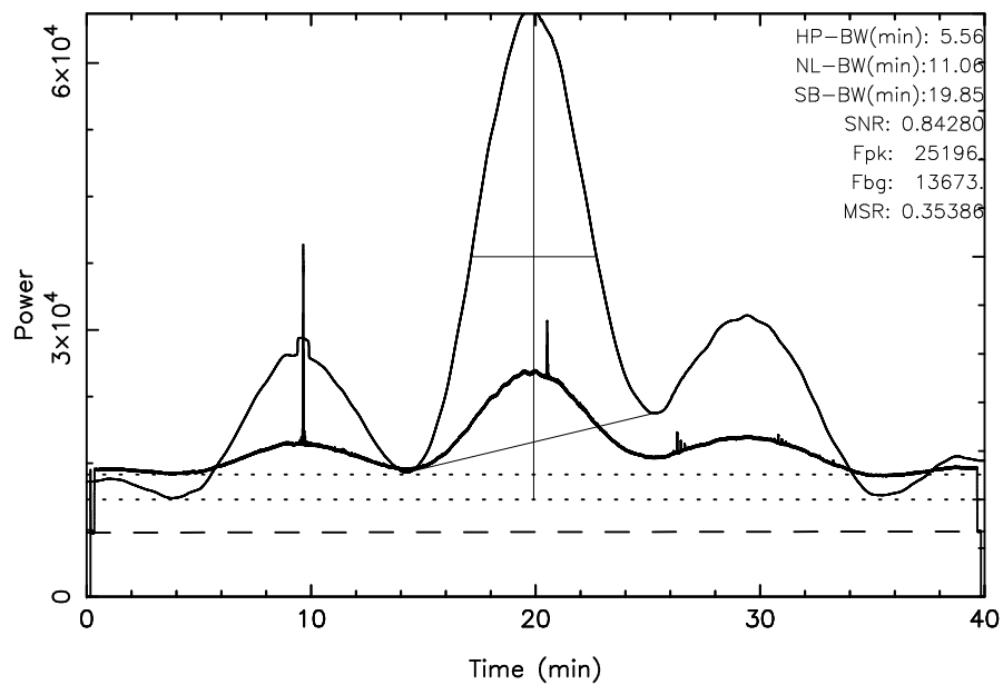
TOYOKAWA 3C144 2025/01/08(008)21:53:11-22:33:11JST
