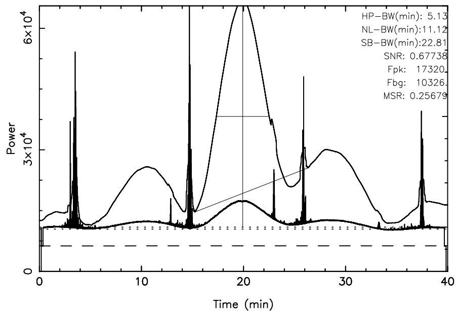
TOYOKAWA 3C274 2025/01/08(008)04:52:02-05:32:02JST
