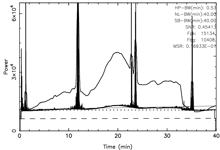
TOYOKAWA 3C123 2025/01/08(008)20:55:58-21:35:58JST
