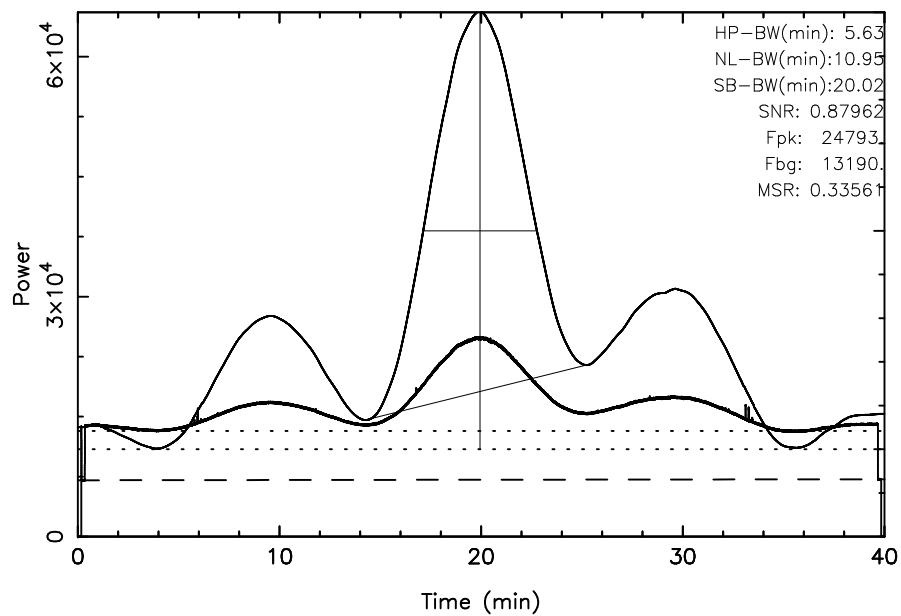
TOYOKAWA 3C144 2025/01/11(011)21:41:23-22:21:23JST
