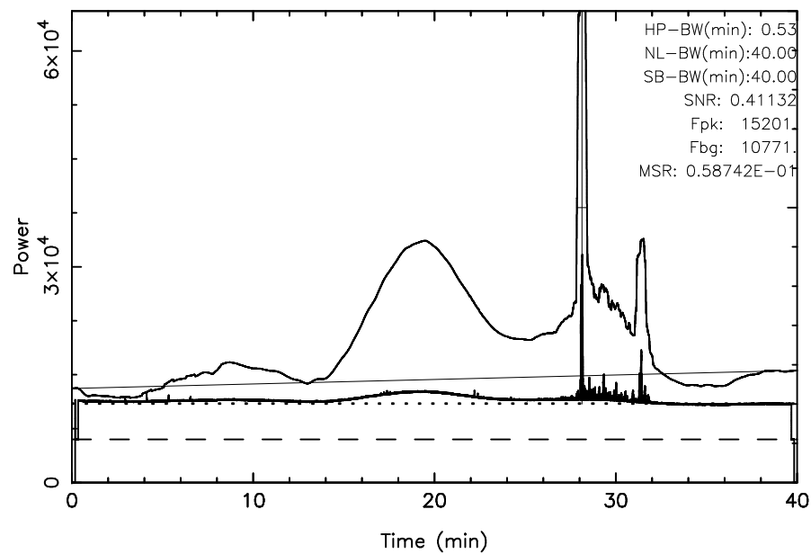
TOYOKAWA 3C157 2025/01/11(011)22:24:47-23:04:47JST
