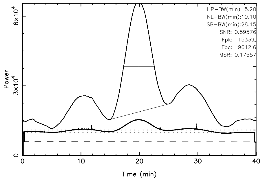
TOYOKAWA 3C274 2025/01/11(011)04:40:15-05:20:15JST
