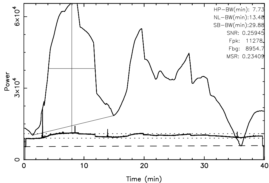
TOYOKAWA 3C123 2025/01/11(011)20:44:10-21:24:10JST
