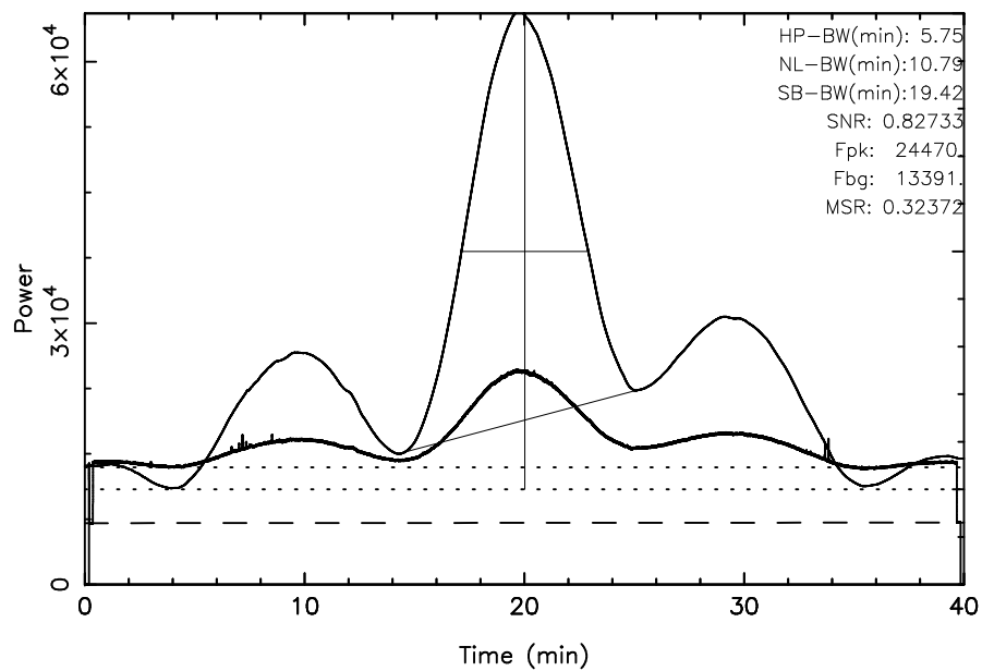
TOYOKAWA 3C144 2025/01/15(015)21:25:39-22:05:39JST
