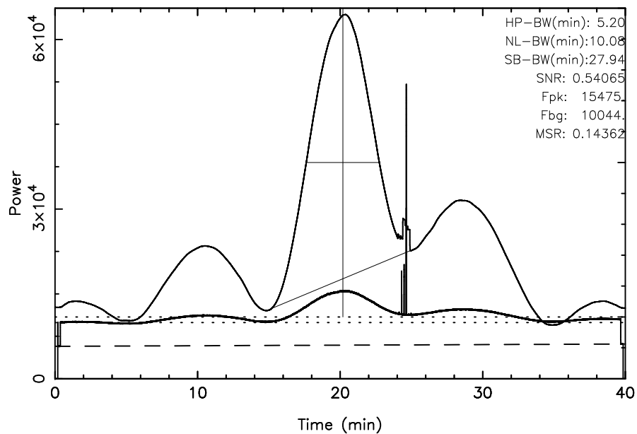
TOYOKAWA 3C274 2025/01/15(015)04:24:31-05:04:31JST
