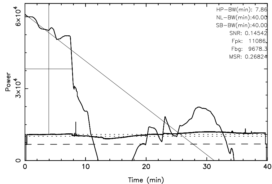
TOYOKAWA 3C123 2025/01/15(015)20:28:27-21:08:27JST
