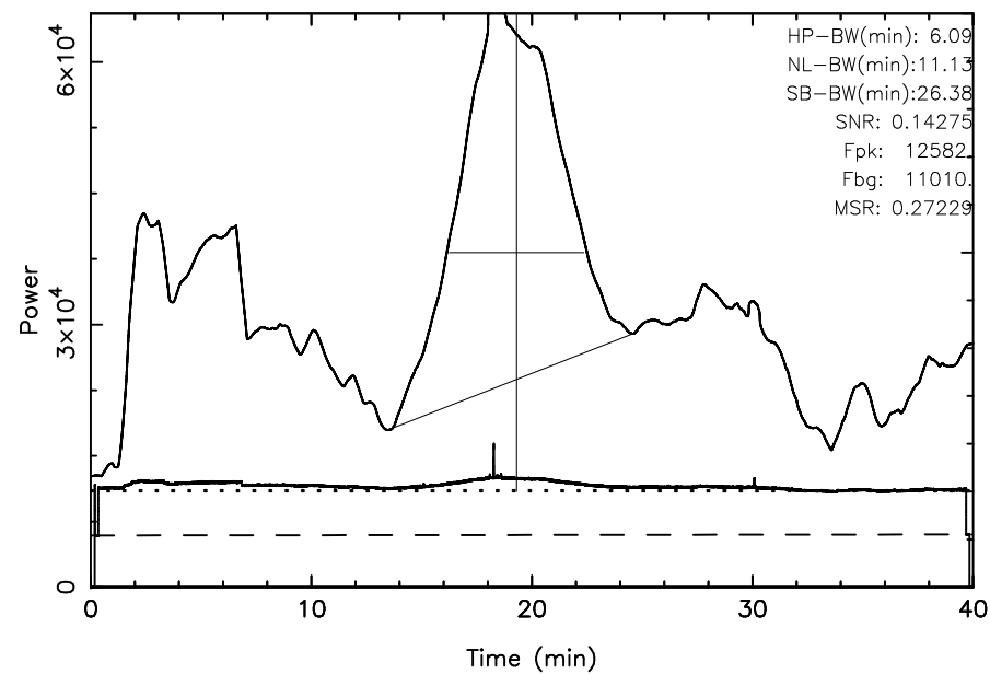
TOYOKAWA 3C157 2025/01/15(015)22:09:04-22:49:04JST
