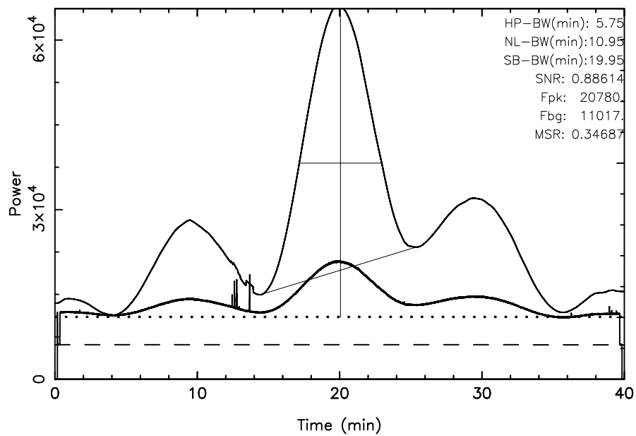
TOYOKAWA 3C144 2025/01/16(016)21:21:43-22:01:43JST
