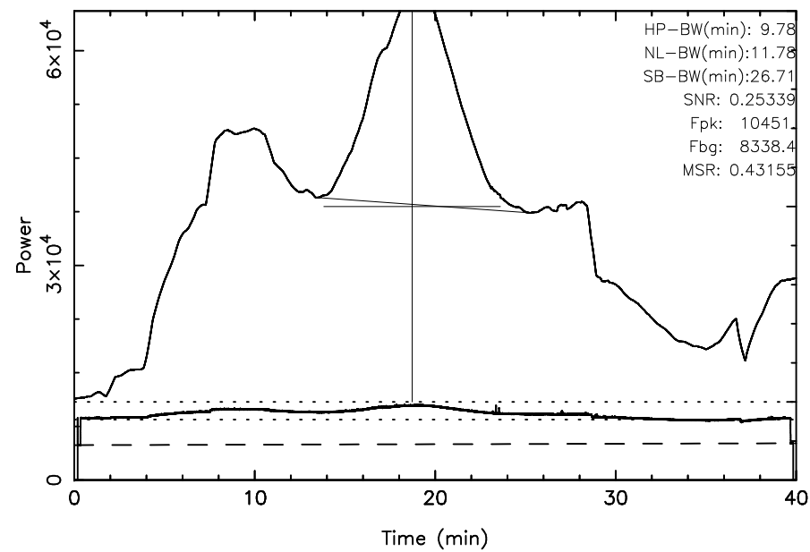
TOYOKAWA 3C157 2025/01/16(016)22:05:08-22:45:08JST
