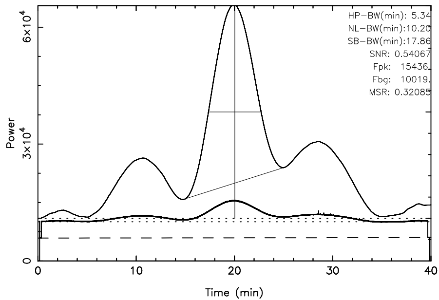
TOYOKAWA 3C274 2025/01/16(016)04:20:35-05:00:35JST
