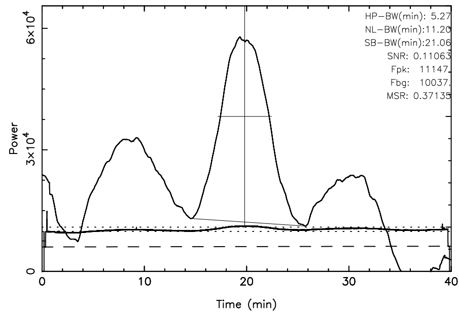
TOYOKAWA 3C123 2025/01/16(016)20:24:31-21:04:31JST
