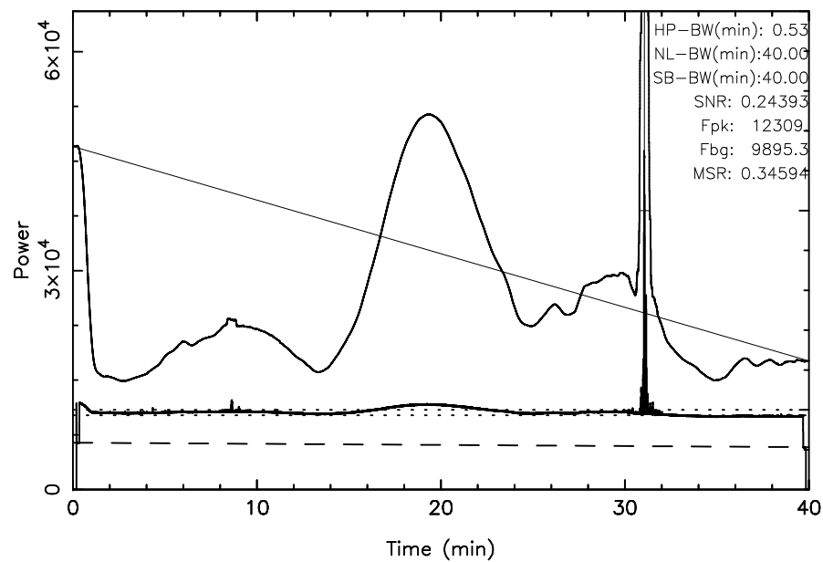
TOYOKAWA 3C157 2025/01/19(019)21:53:20-22:33:20JST
