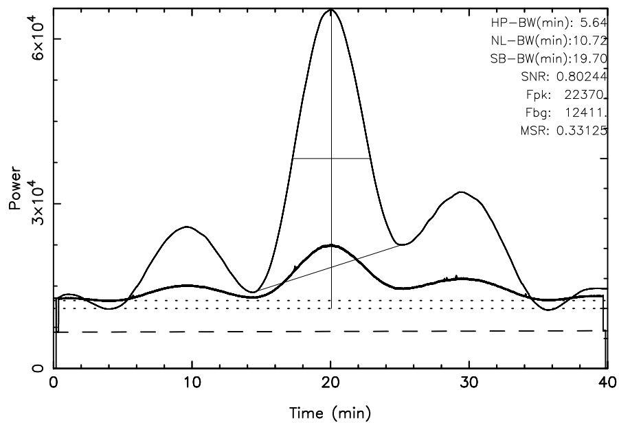
TOYOKAWA 3C144 2025/01/19(019)21:09:56-21:49:56JST
