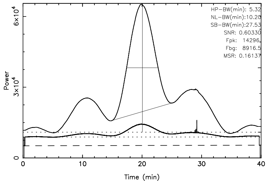
TOYOKAWA 3C274 2025/01/19(019)04:08:47-04:48:47JST
