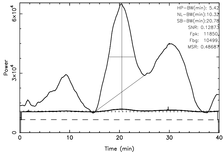
TOYOKAWA 3C123 2025/01/19(019)20:12:43-20:52:43JST
