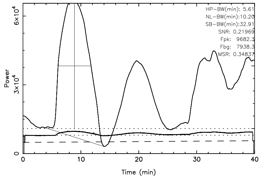
TOYOKAWA 3C123 2025/01/21(021)20:04:51-20:44:51JST
