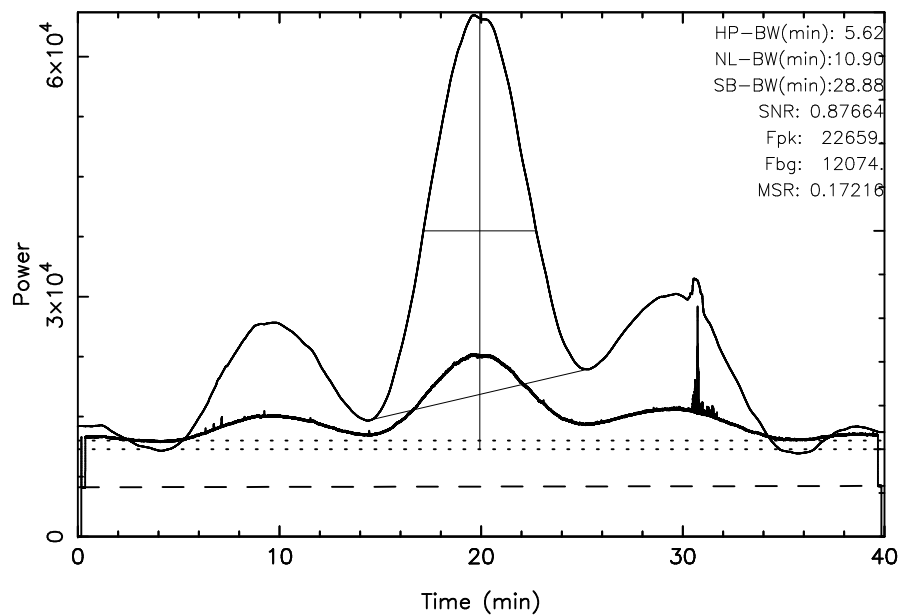
TOYOKAWA 3C144 2025/01/21(021)21:02:04-21:42:04JST
