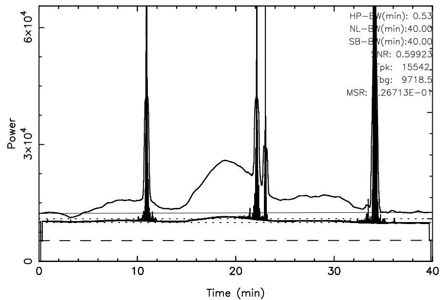
TOYOKAWA 3C157 2025/01/21(021)21:45:28-22:25:28JST
