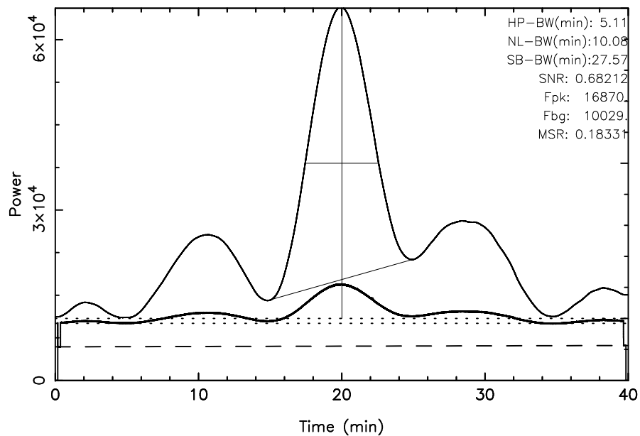
TOYOKAWA 3C274 2025/01/21(021)04:00:56-04:40:56JST
