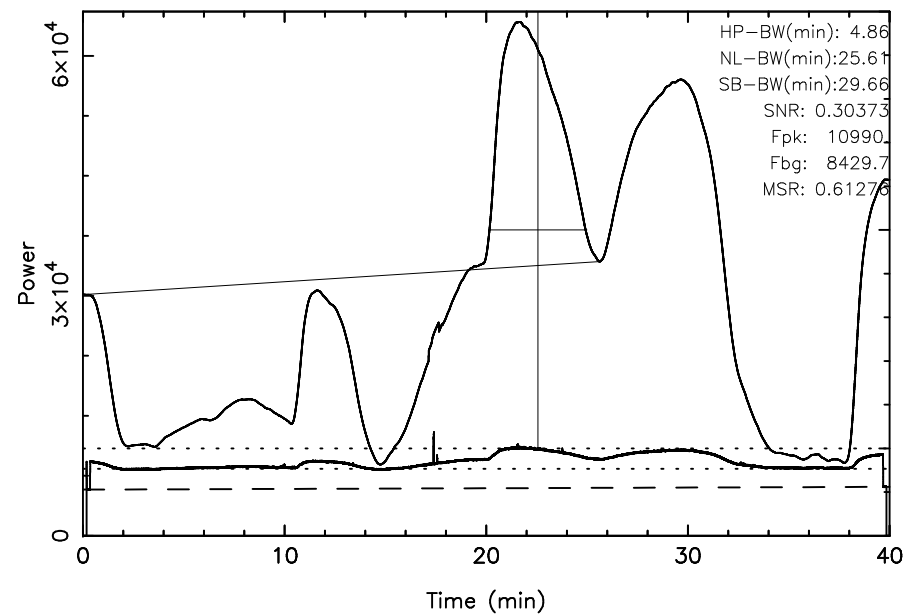
TOYOKAWA 3C123 2025/01/22(022)20:00:56-20:40:56JST
