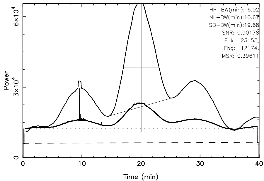
TOYOKAWA 3C144 2025/01/22(022)20:58:08-21:38:08JST
