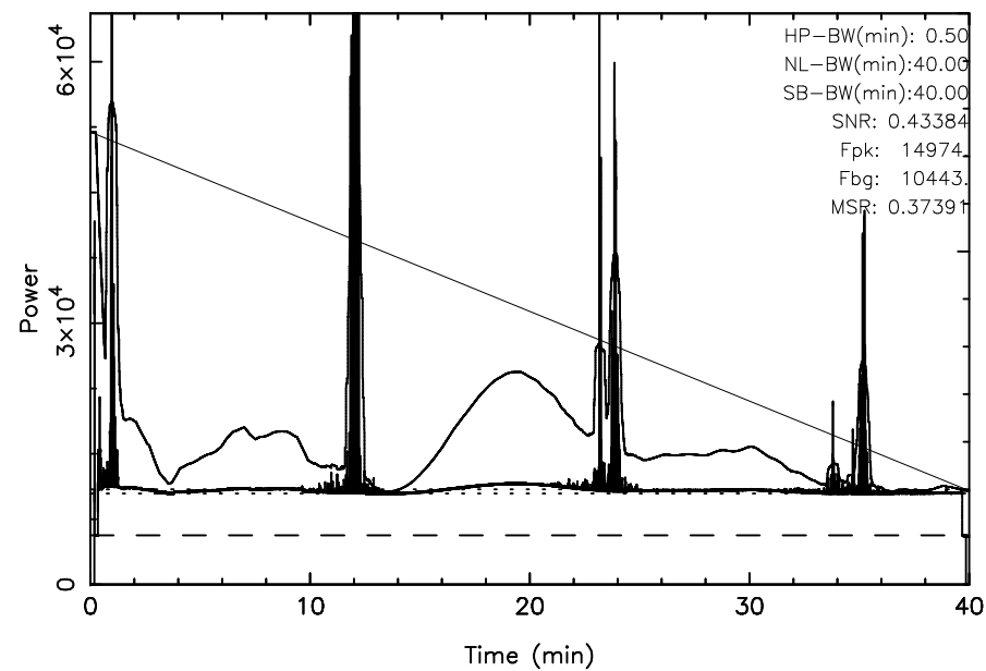
TOYOKAWA 3C157 2025/01/22(022)21:41:32-22:21:32JST
