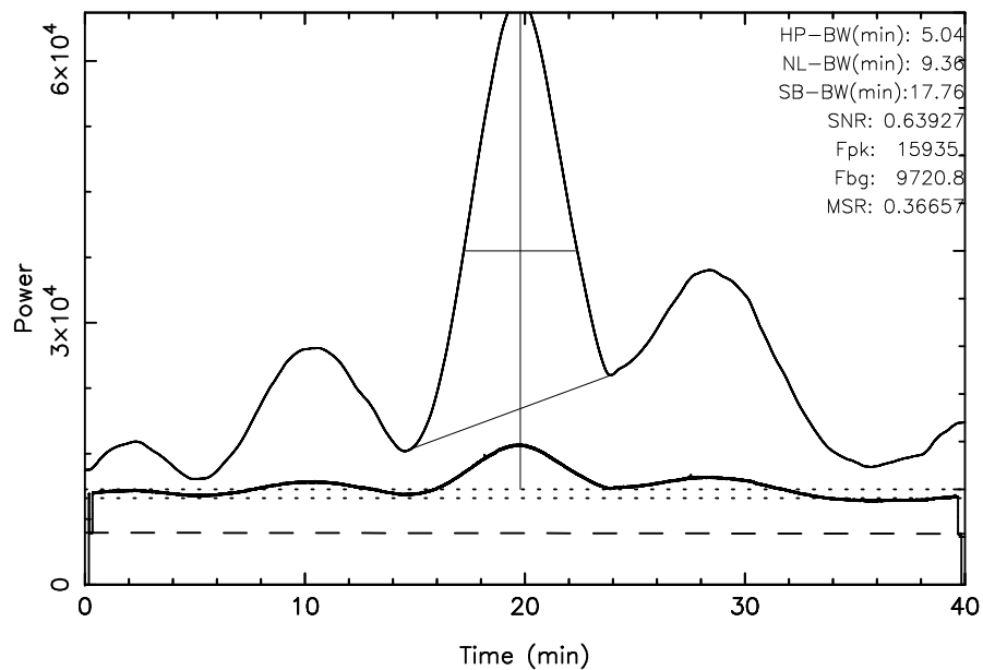
TOYOKAWA 3C274 2025/01/22(022)03:57:00-04:37:00JST
