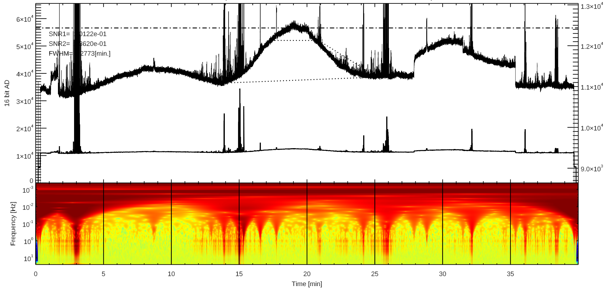
C 3C157 (/home4/archive/swift/dat/2025/02/T20250220194733.dat)
