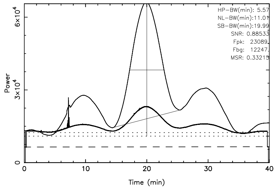
TOYOKAWA 3C144 2025/02/01(032)20:18:49-20:58:49JST
