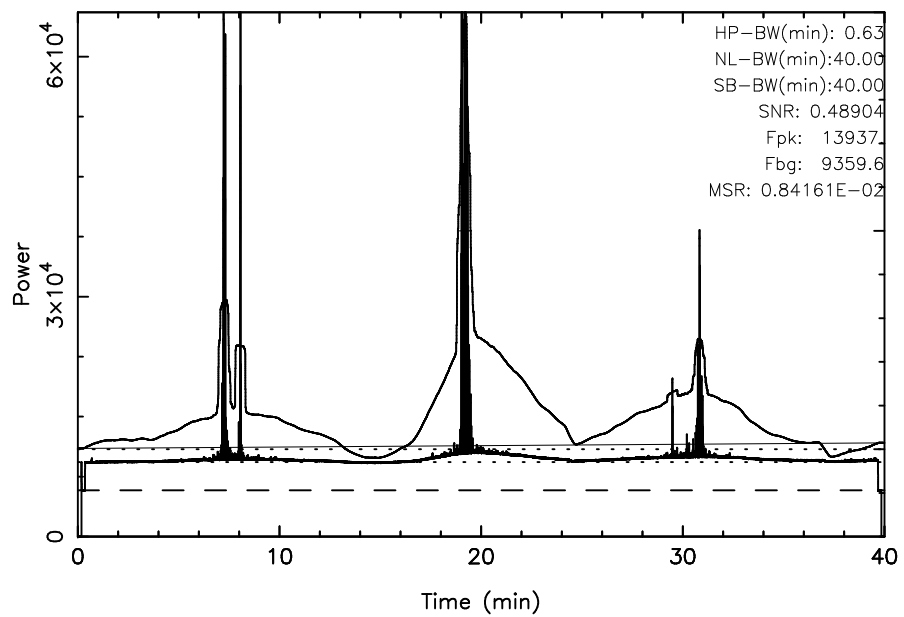
TOYOKAWA 3C123 2025/02/01(032)19:21:37-20:01:37JST
