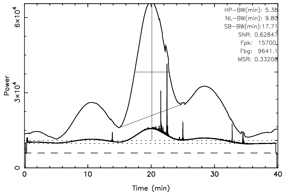
TOYOKAWA 3C274 2025/02/01(032)03:17:41-03:57:41JST
