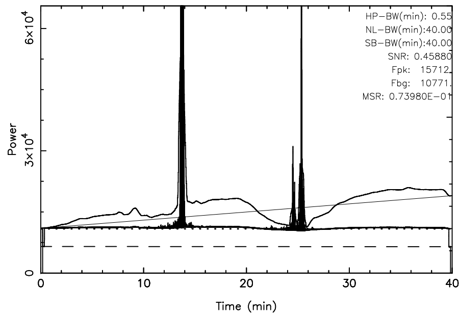
TOYOKAWA 3C295 2025/02/01(032)04:57:32-05:37:32JST
