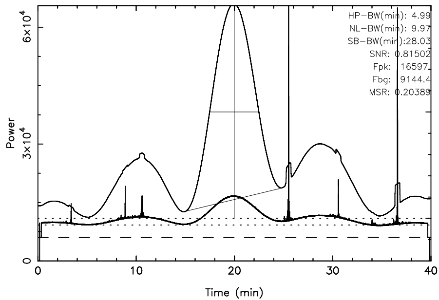
TOYOKAWA 3C274 2025/02/02(033)03:13:45-03:53:45JST
