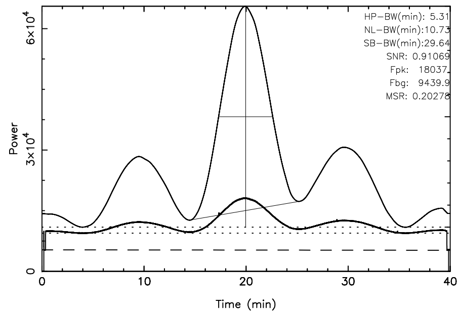
TOYOKAWA 3C144 2025/02/02(033)20:14:53-20:54:53JST
