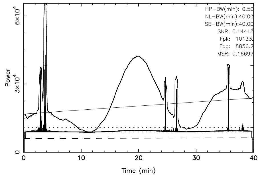
TOYOKAWA 3C295 2025/02/02(033)04:53:36-05:33:36JST
