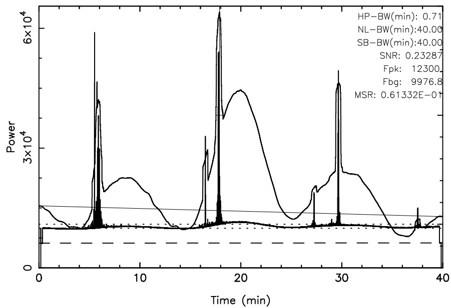
TOYOKAWA 3C123 2025/02/02(033)19:17:41-19:57:41JST
