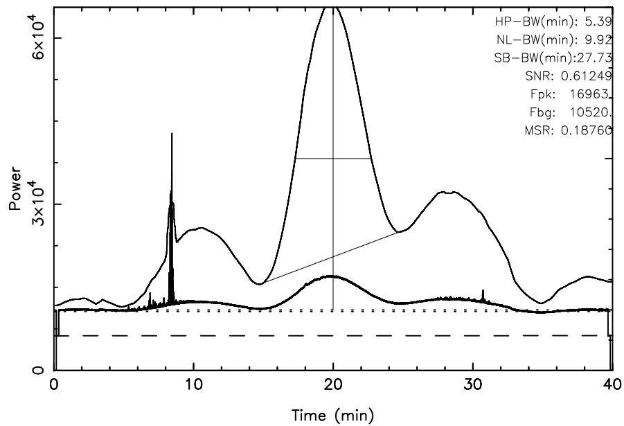
TOYOKAWA 3C274 2025/02/08(039)02:50:09-03:30:09JST
