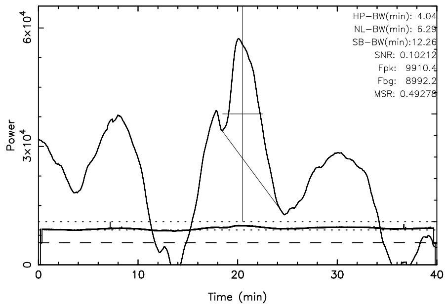
TOYOKAWA 3C123 2025/02/11(042)18:42:18-19:22:18JST
