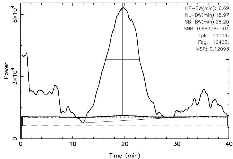
TOYOKAWA 3C295 2025/02/11(042)04:18:13-04:58:13JST
