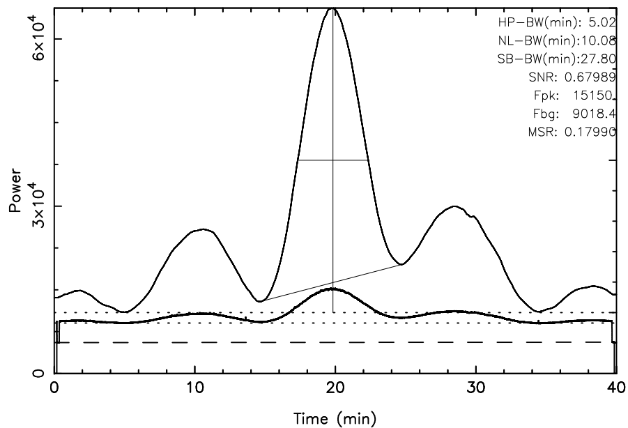
TOYOKAWA 3C274 2025/02/11(042)02:38:22-03:18:22JST
