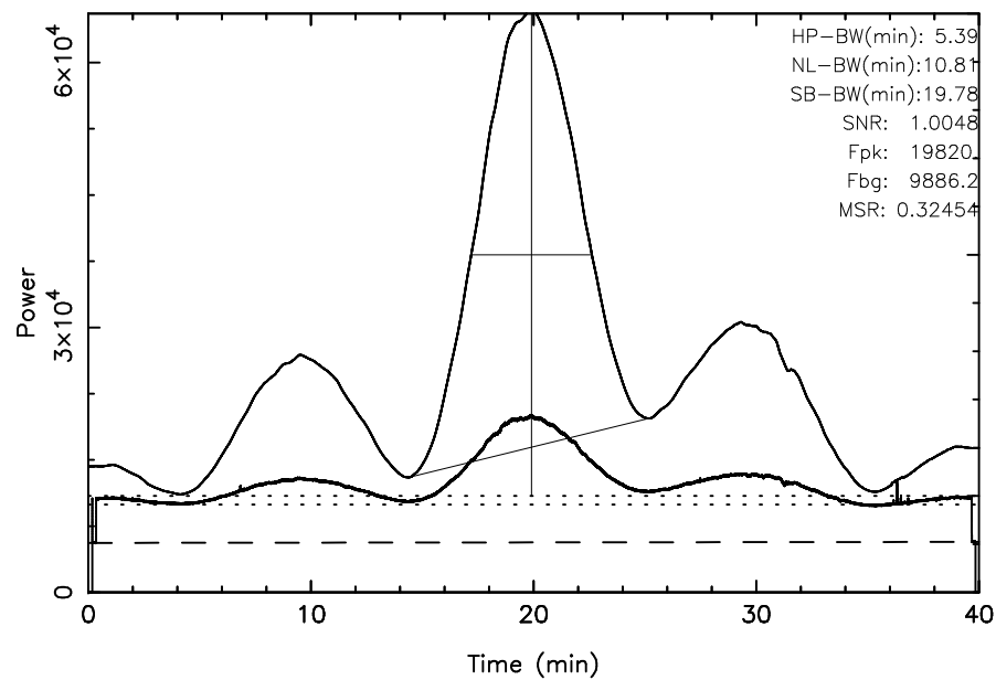
TOYOKAWA 3C144 2025/02/11(042)19:39:30-20:19:30JST
