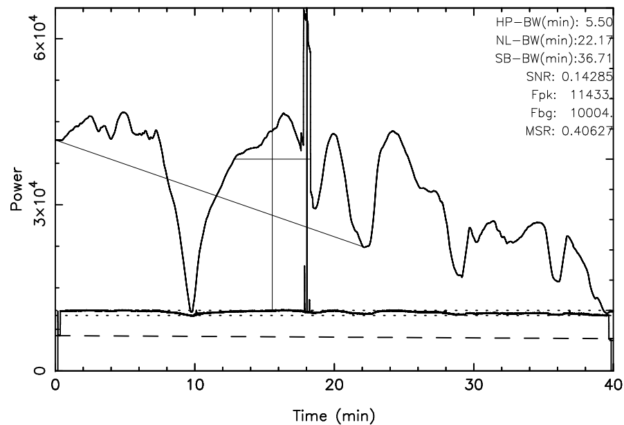
TOYOKAWA 3C295 2025/02/12(043)04:14:17-04:54:17JST
