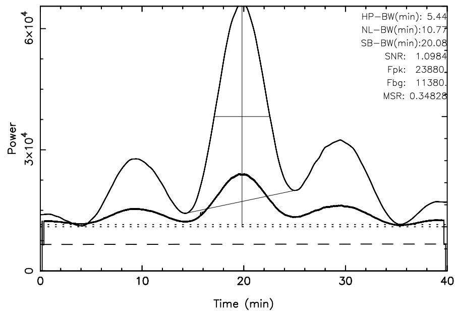
TOYOKAWA 3C144 2025/02/12(043)19:35:34-20:15:34JST
