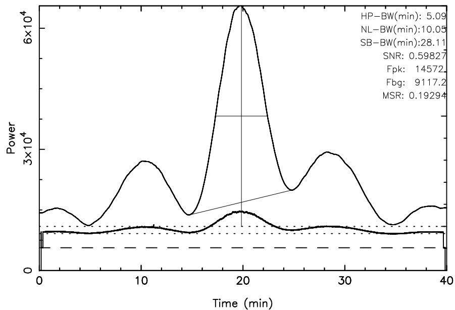
TOYOKAWA 3C274 2025/02/12(043)02:34:26-03:14:26JST
