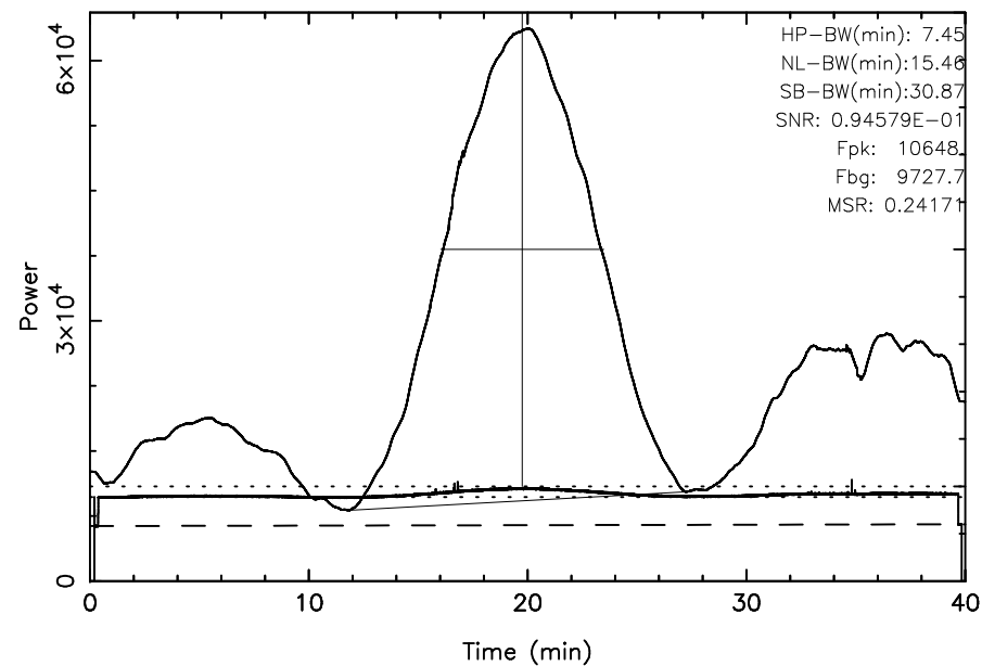
TOYOKAWA 3C295 2025/02/13(044)04:10:21-04:50:21JST
