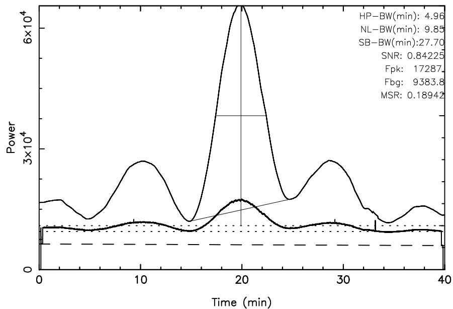
TOYOKAWA 3C274 2025/02/13(044)02:30:30-03:10:30JST
