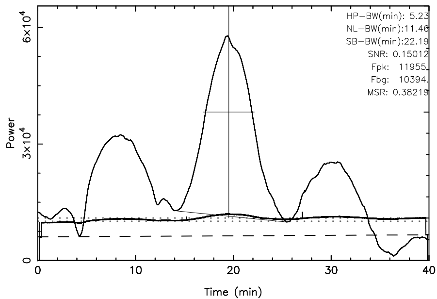
TOYOKAWA 3C123 2025/02/13(044)18:34:26-19:14:26JST
