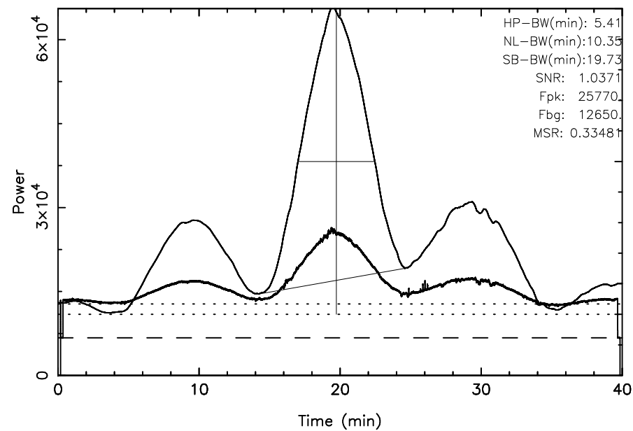
TOYOKAWA 3C144 2025/02/13(044)19:31:38-20:11:38JST
