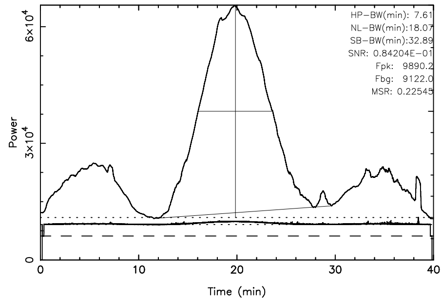
TOYOKAWA 3C295 2025/02/16(047)03:58:34-04:38:34JST
