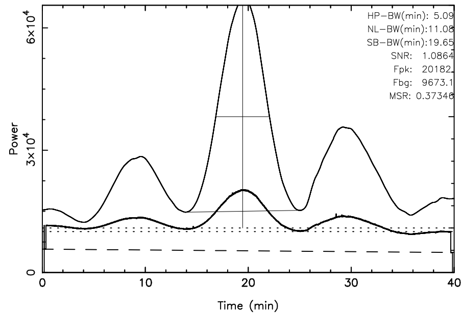
TOYOKAWA 3C144 2025/02/16(047)19:19:51-19:59:51JST
