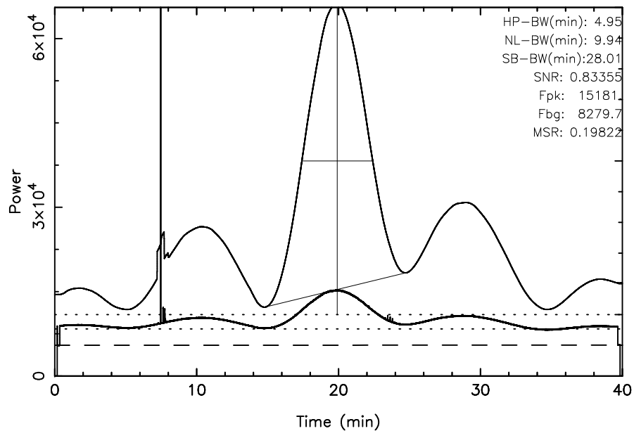
TOYOKAWA 3C274 2025/02/16(047)02:18:42-02:58:42JST
