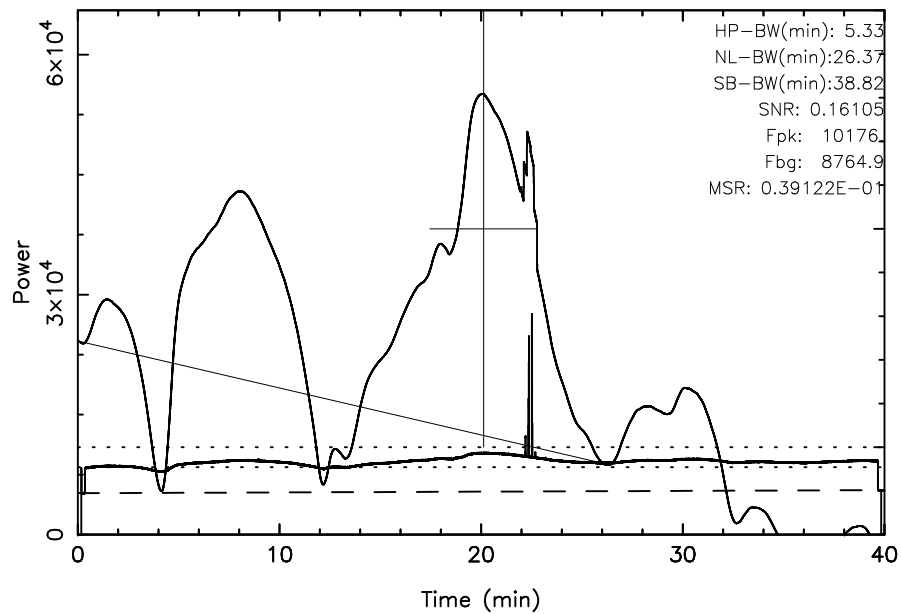
TOYOKAWA 3C123 2025/02/16(047)18:22:38-19:02:38JST
