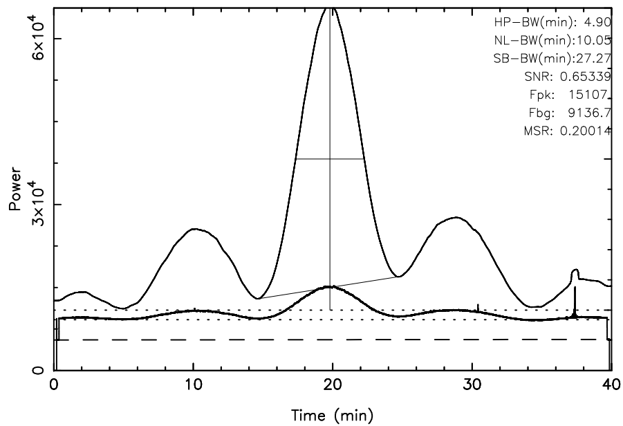
TOYOKAWA 3C274 2025/02/19(050)02:06:54-02:46:54JST
