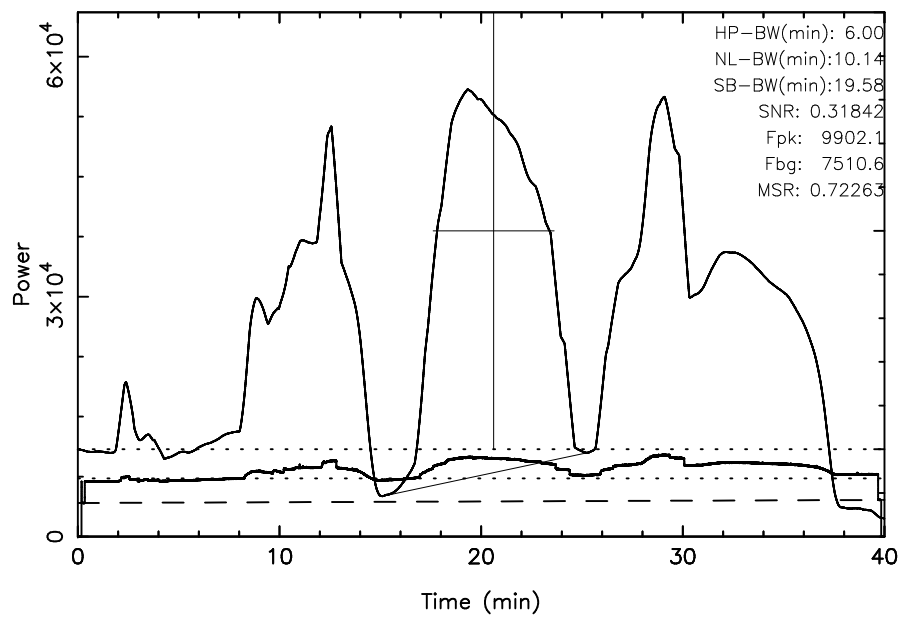
TOYOKAWA 3C123 2025/02/19(050)18:10:50-18:50:50JST
