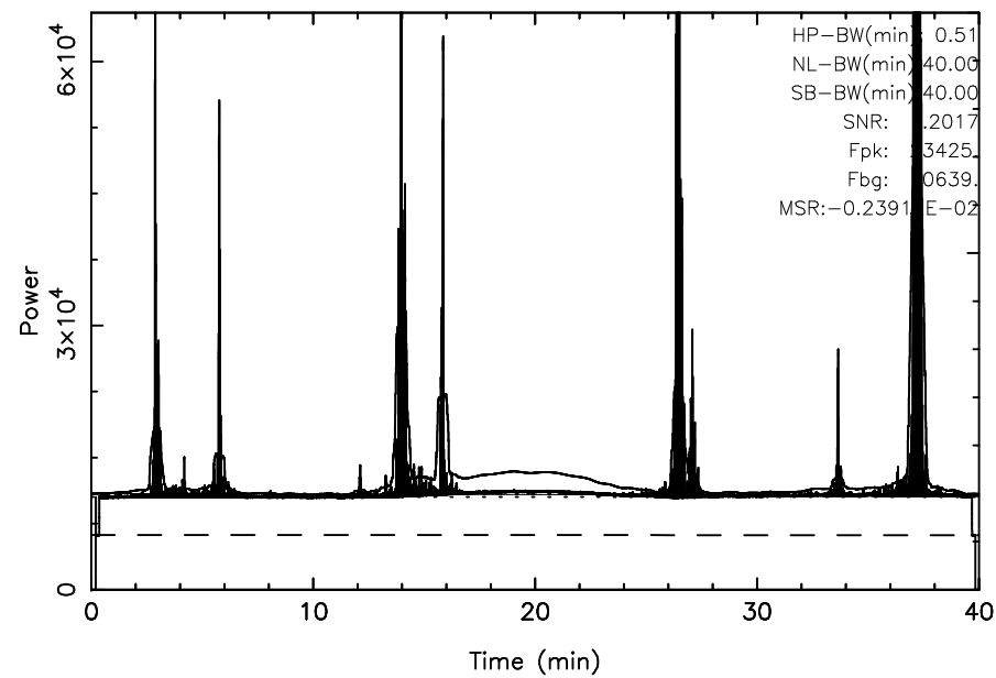
TOYOKAWA 3C295 2025/02/19(050)03:46:46-04:26:46JST
