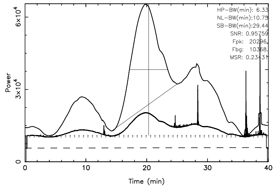
TOYOKAWA 3C144 2025/02/19(050)19:08:03-19:48:03JST
