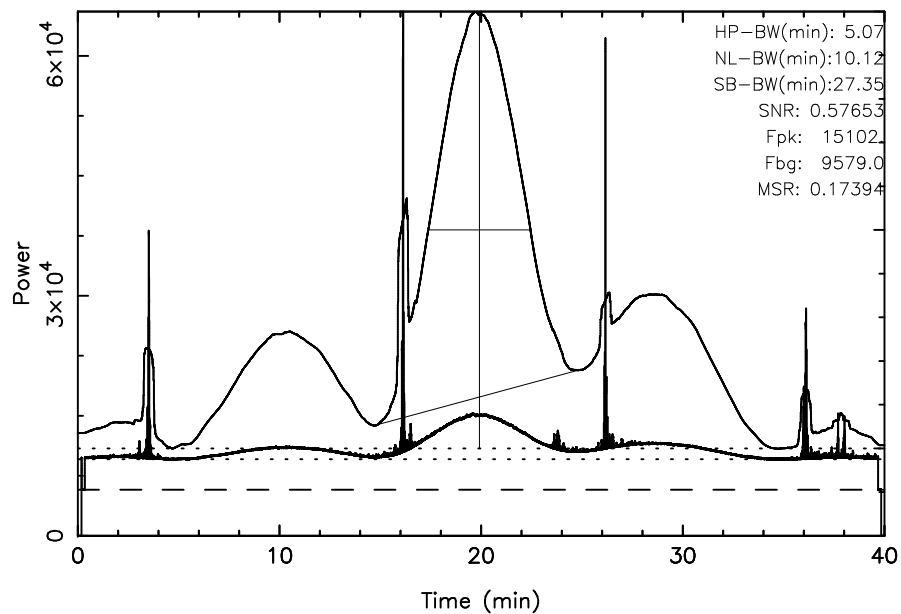
TOYOKAWA 3C274 2025/02/22(053)01:55:07-02:35:07JST
