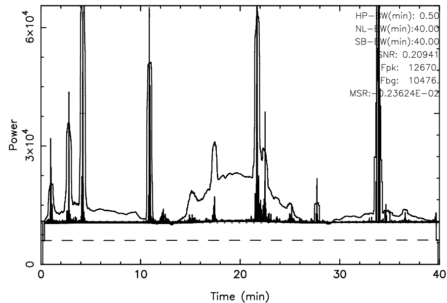
TOYOKAWA 3C295 2025/02/22(053)03:34:58-04:14:58JST
