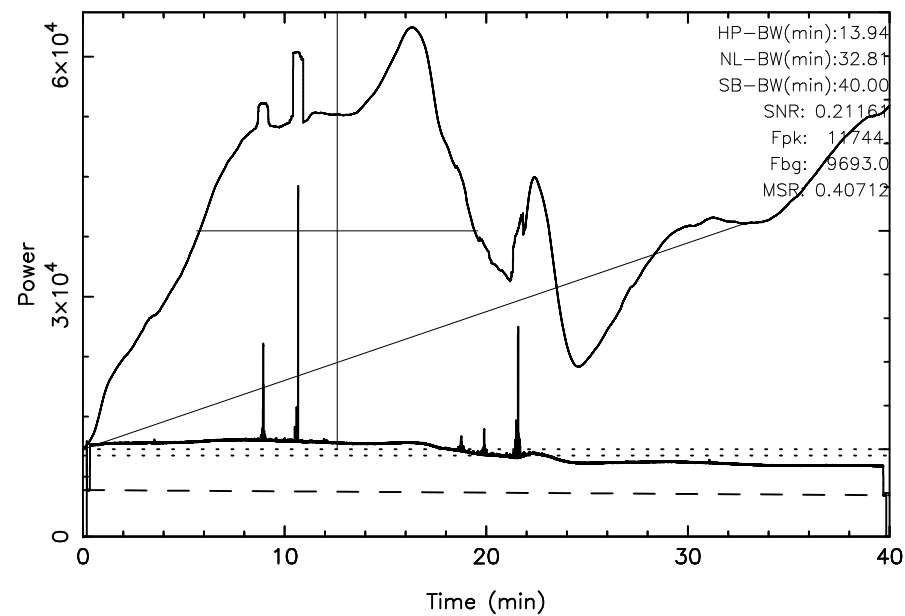
TOYOKAWA 3C157 2025/02/22(053)19:39:40-20:19:40JST
