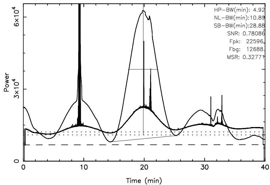
TOYOKAWA 3C144 2025/02/22(053)18:56:15-19:36:15JST
