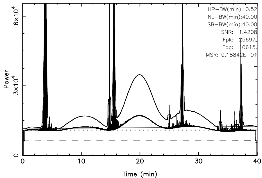
TOYOKAWA 3C274 2025/02/25(056)01:43:19-02:23:19JST
