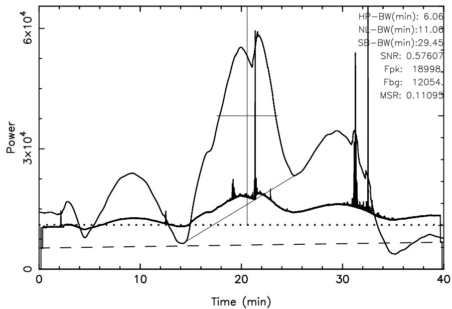
TOYOKAWA 3C144 2025/02/25(056)18:44:27-19:24:27JST
