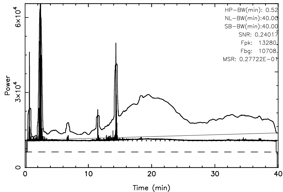
TOYOKAWA 3C295 2025/02/25(056)03:23:10-04:03:10JST
