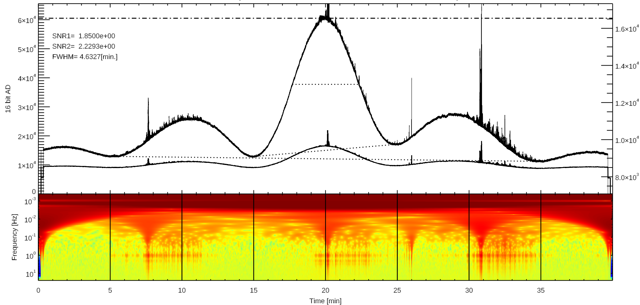
C 3C274 (/home4/archive/swift/dat/2025/03/T20250317002443.dat)
