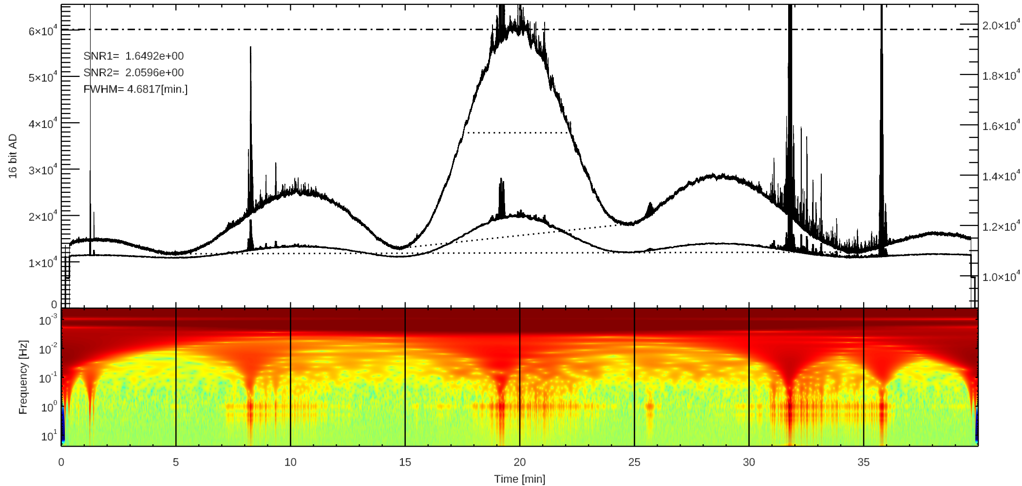
C 3C274 (/home4/archive/swift/dat/2025/03/T20250318002047.dat)
