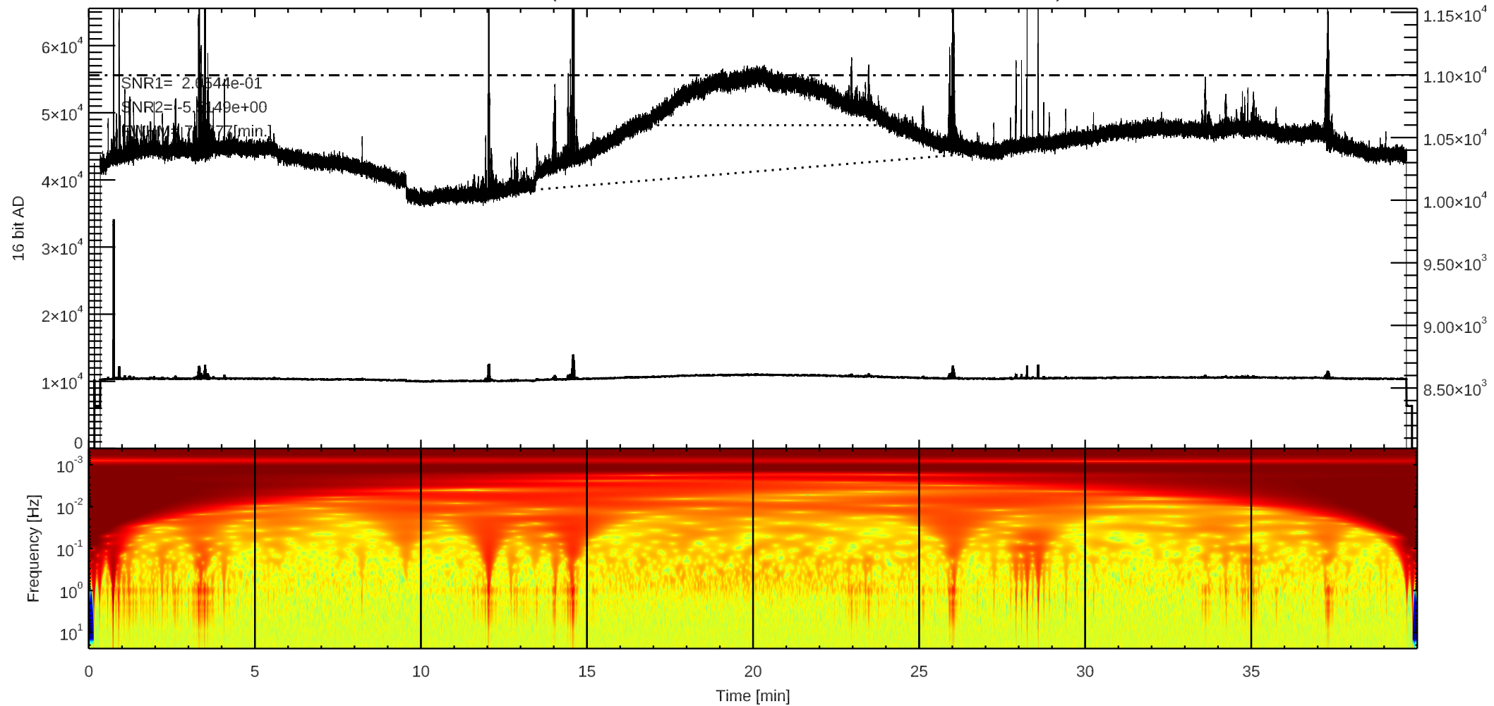
C 3C295 (/home4/archive/swift/dat/2025/03/T20250323014059.dat)
