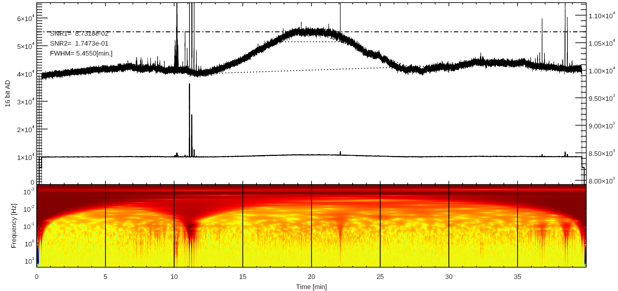
C 3C295 (/home4/archive/swift/dat/2025/03/T20250325013307.dat)
