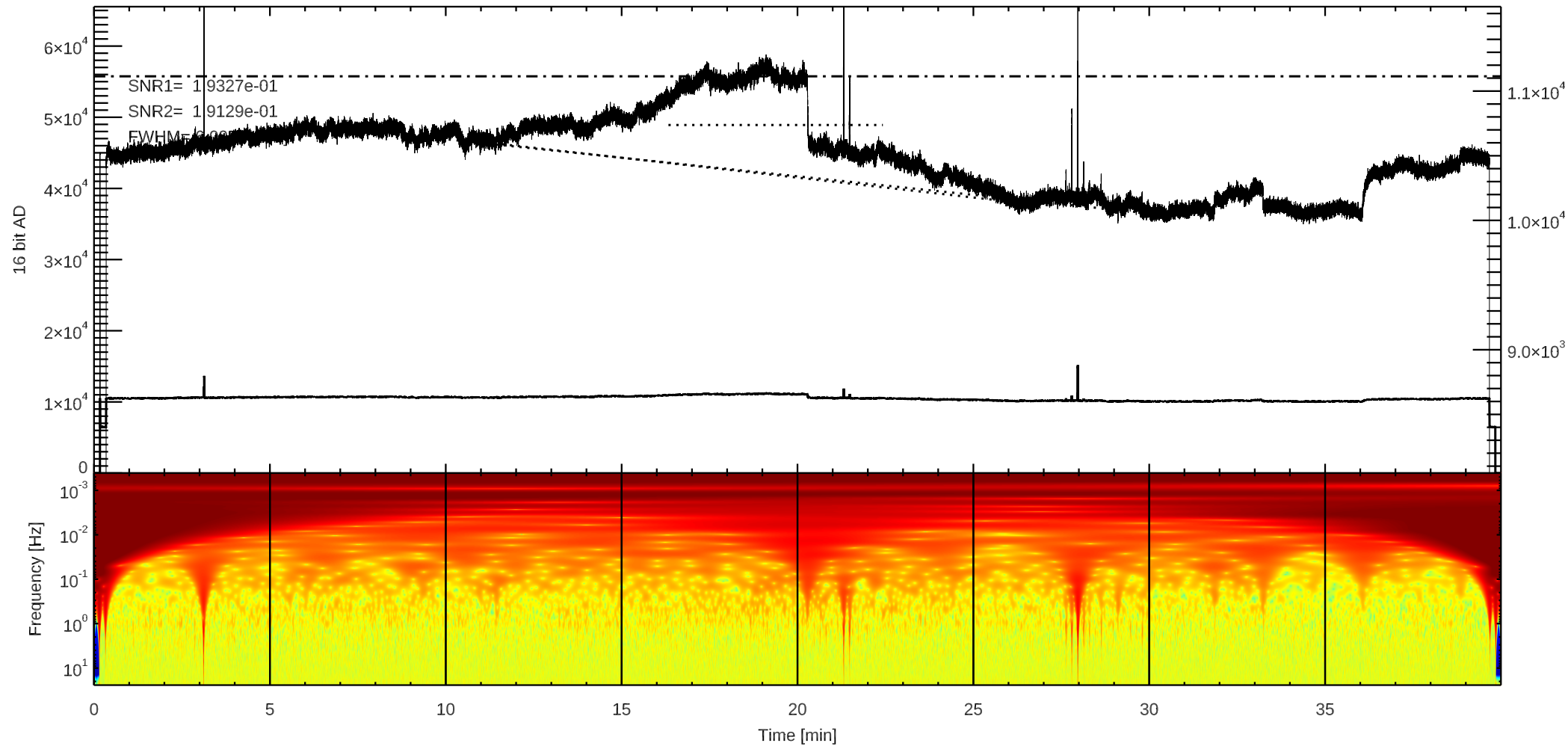
C 3C295 (/home4/archive/swift/dat/2025/03/T20250327012515.dat)
