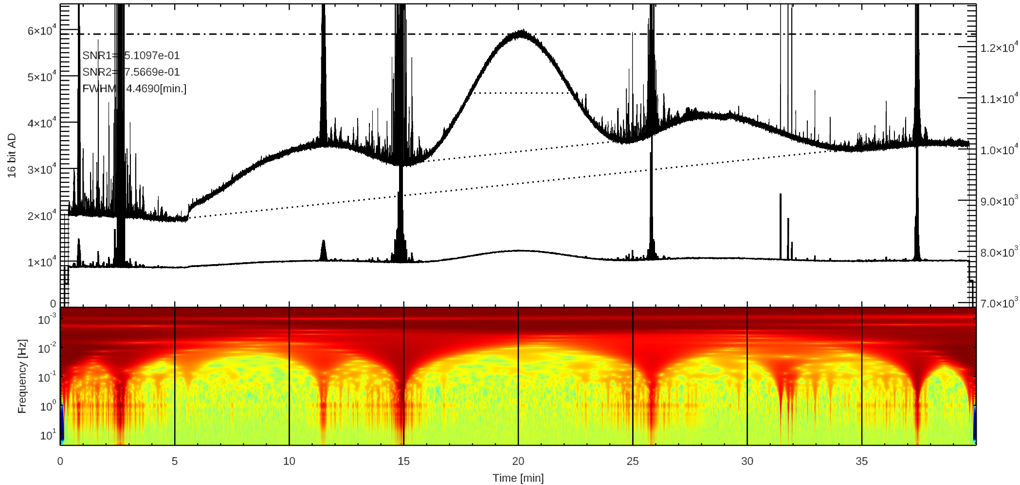
C 3C348 (/home4/archive/swift/dat/2025/03/T20250312050357.dat)
