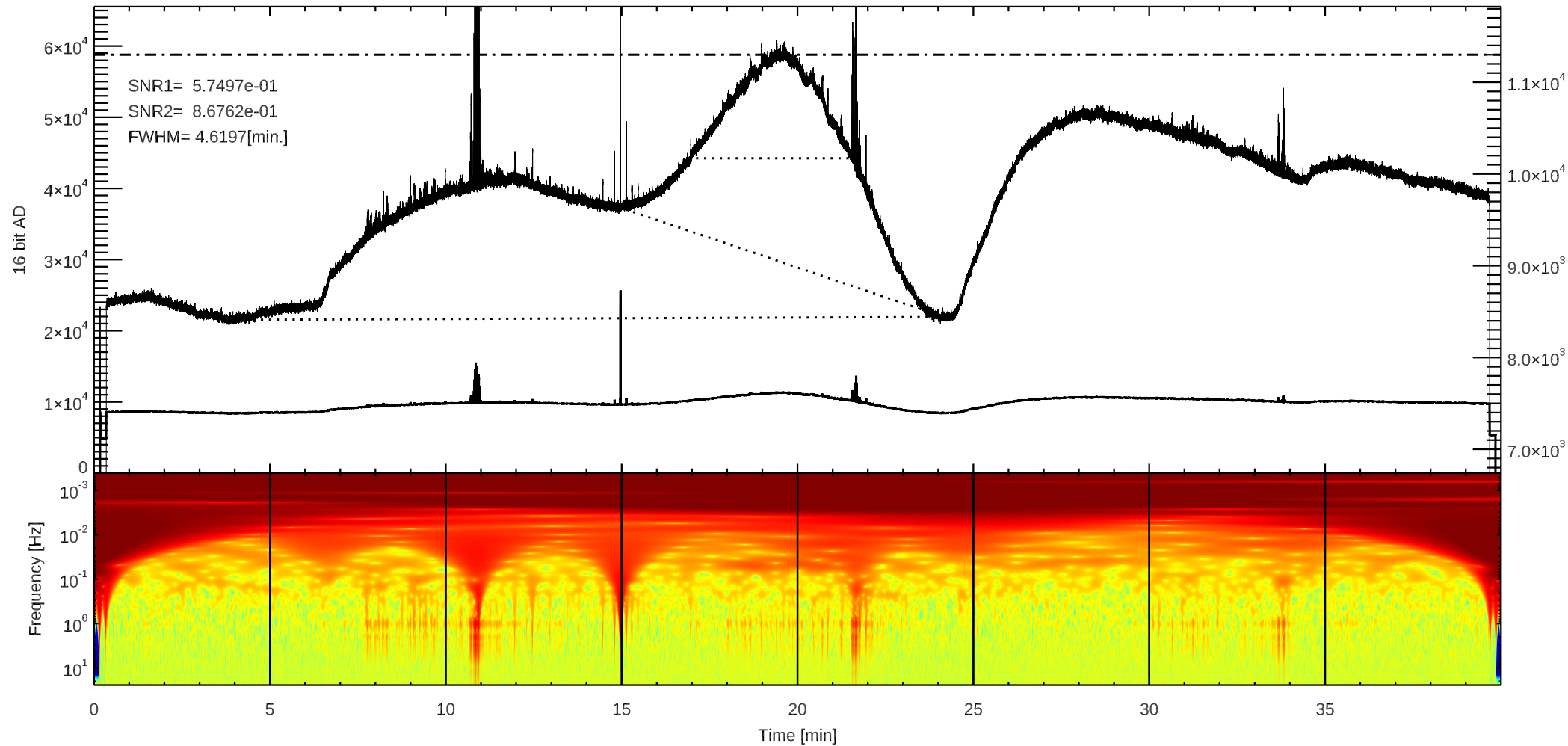
C 3C348 (/home4/archive/swift/dat/2025/03/T20250314045606.dat)
